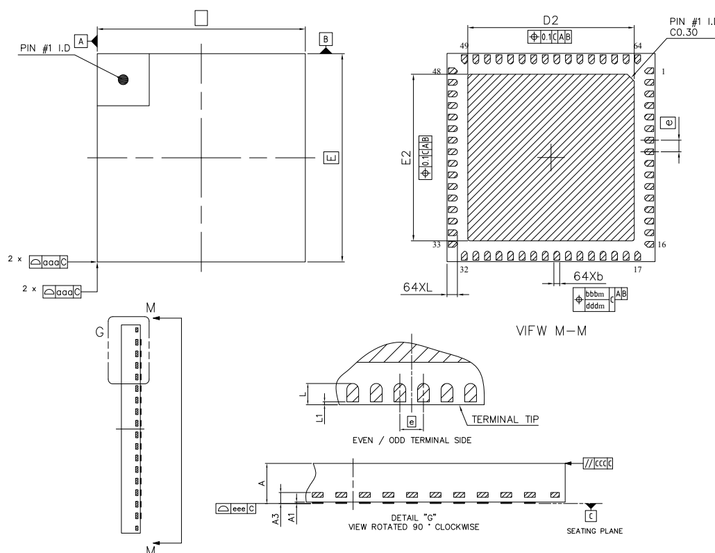
Figure 10.1. QFN64
