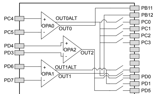
Figure 5.40. Opamp Pinout
