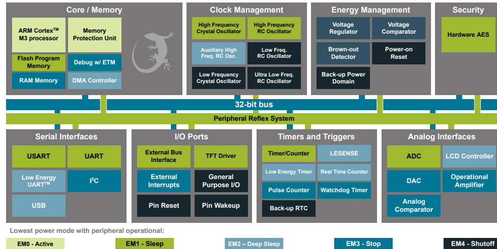
Figure 3.1. Block Diagram
