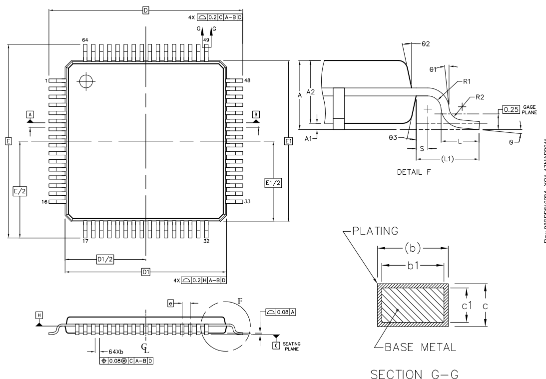
Figure 11.1. TQFP64
