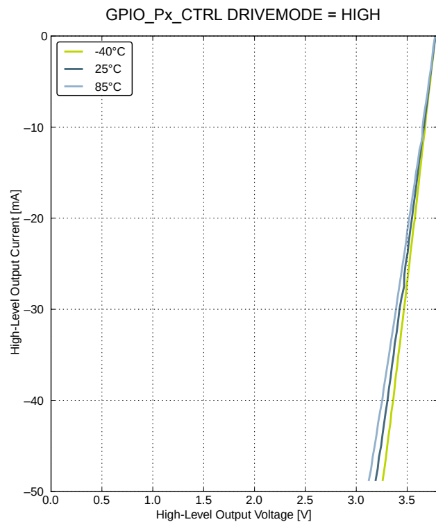
Figure 4.16. Typical High-Level Output Current, 3.8 V Supply Voltage
