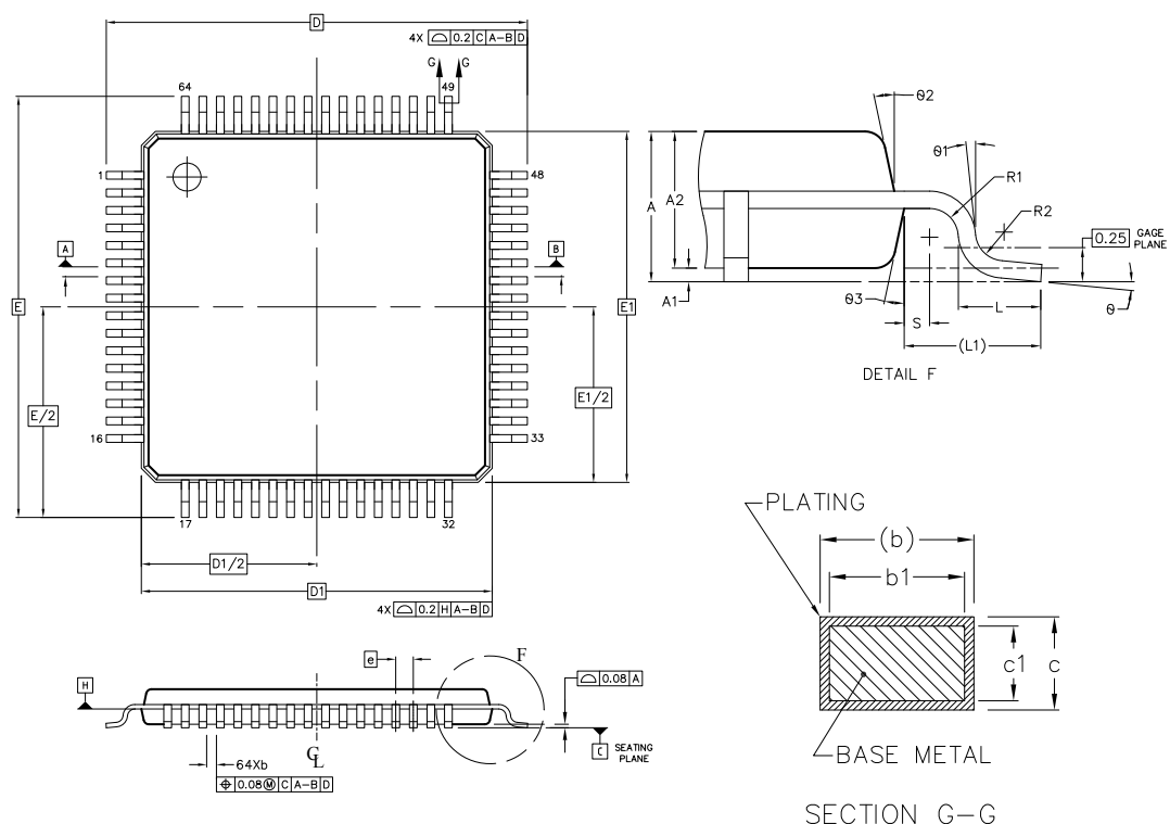
Figure 11.1. TQFP64
