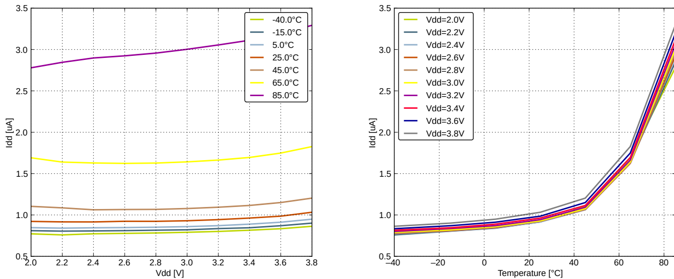
Figure 4.8. EM2 Current Consumption, RTC 1 prescaled to 1 kHz, 32.768 kHz LFRCO
