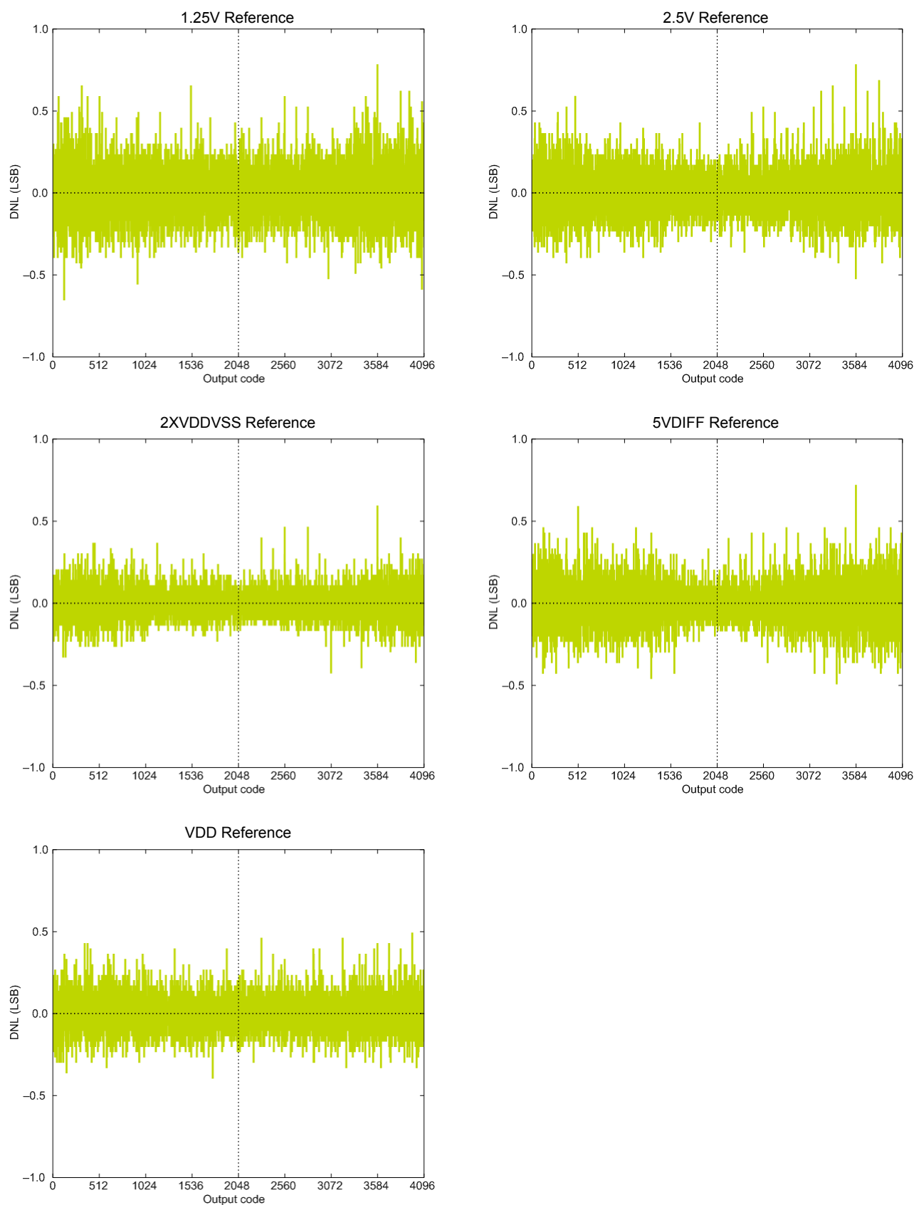
Figure 4.28. ADC Differential Linearity Error vs Code, VDD = 3 V, Temp = 25 °C
