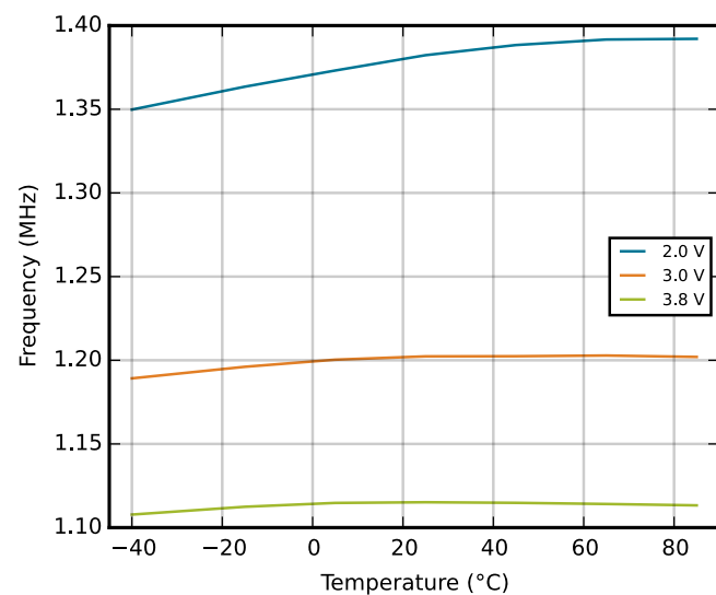
Figure 4.18. Calibrated HFRCO 1 MHz Band Frequency vs Supply Voltage and Temperature
