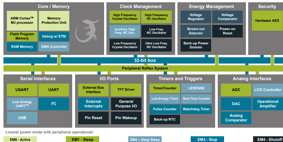
Figure 3.1. Block Diagram
