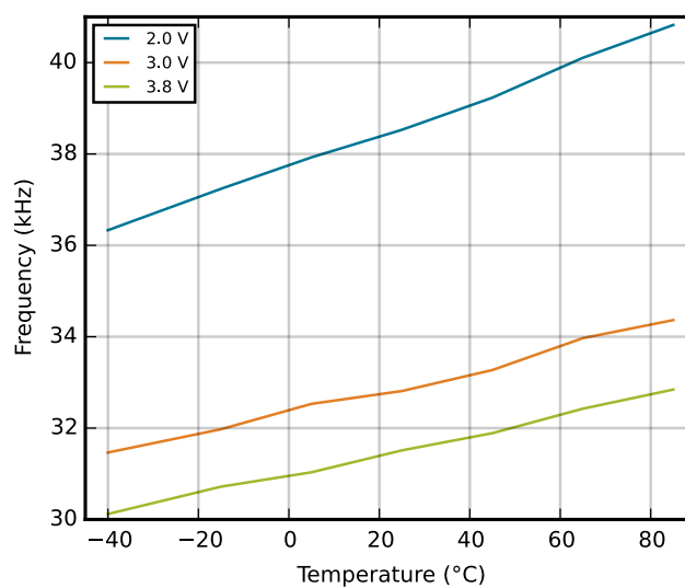
Figure 4.17. Calibrated LFRCO Frequency vs Temperature and Supply Voltage
