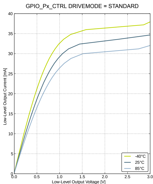
Figure 4.13. Typical Low-Level Output Current, 3 V Supply Voltage
