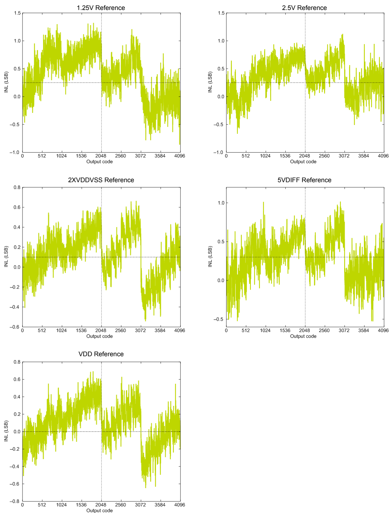
Figure 4.27. ADC Integral Linearity Error vs Code, VDD = 3 V, Temp = 25 °C
