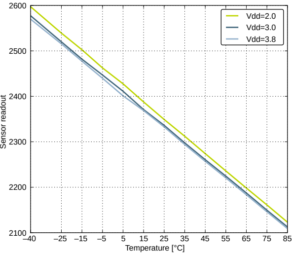
Figure 4.31. ADC Temperature Sensor Readout
