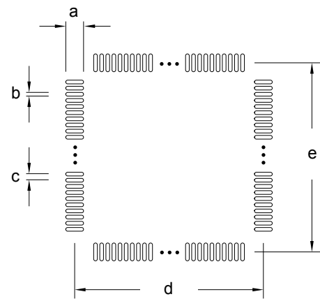
Figure 9.4. LQFP100 PCB Stencil Design
