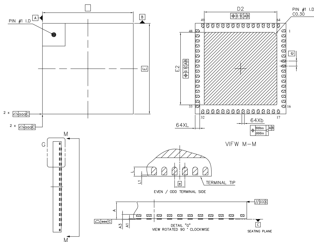
Figure 11.1. QFN64
