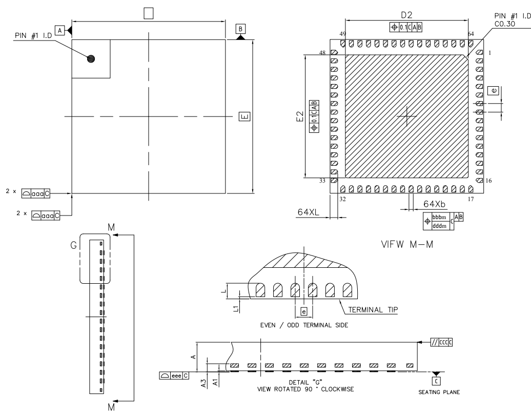
Figure 11.1. QFN64
