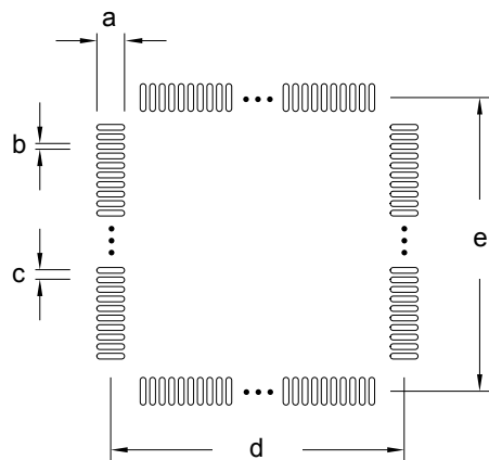
Figure 9.4. LQFP100 PCB Stencil Design
