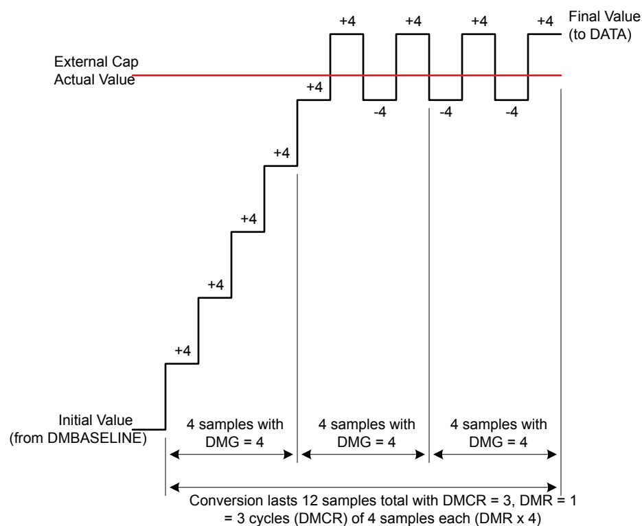
Figure 34.3. Delta Modulation Conversion With Fixed Delta Step (DMCFG_DMGLIS = 1)
