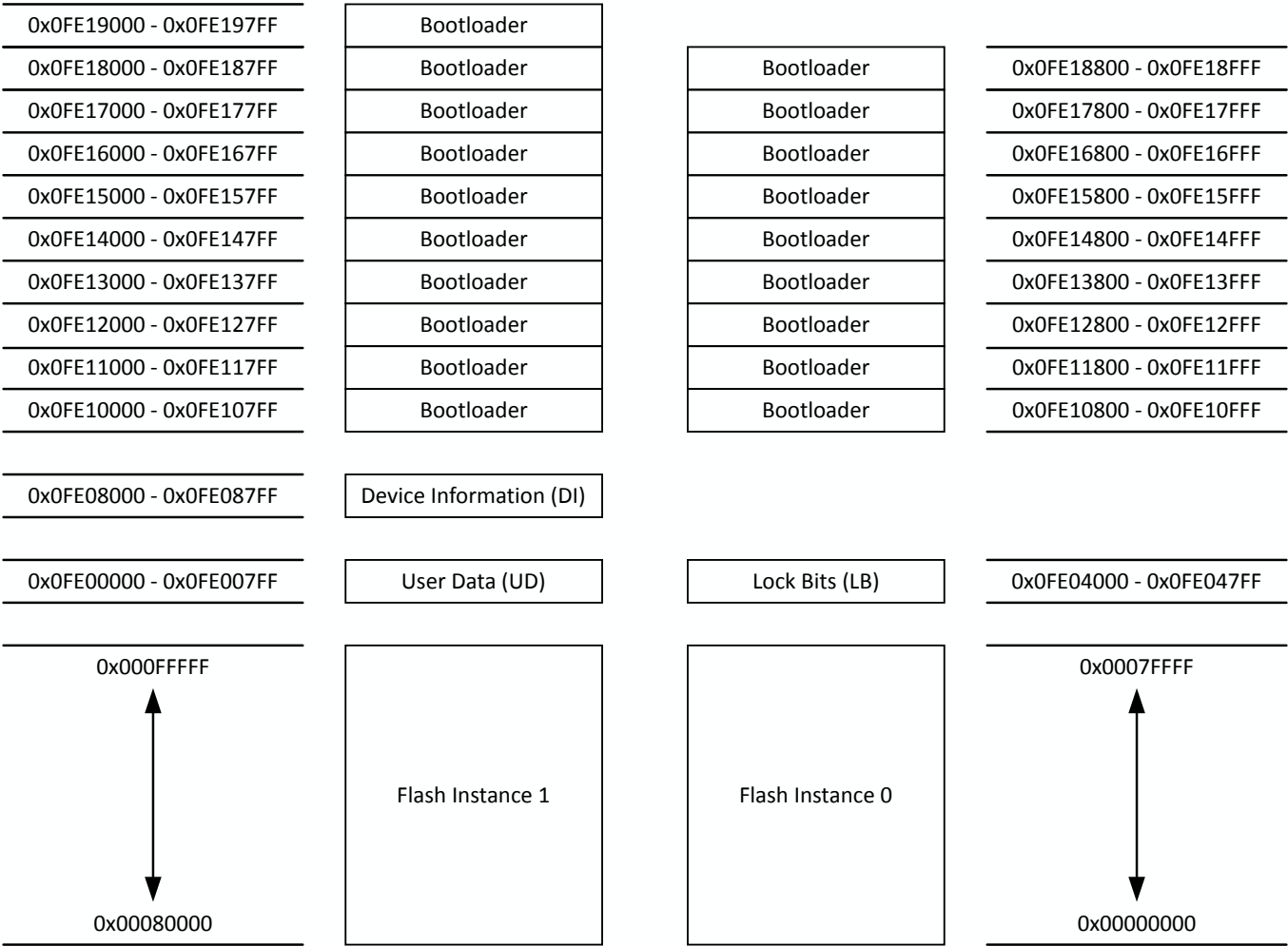
Figure 7.2. Flash Page Organization and Instance Association
