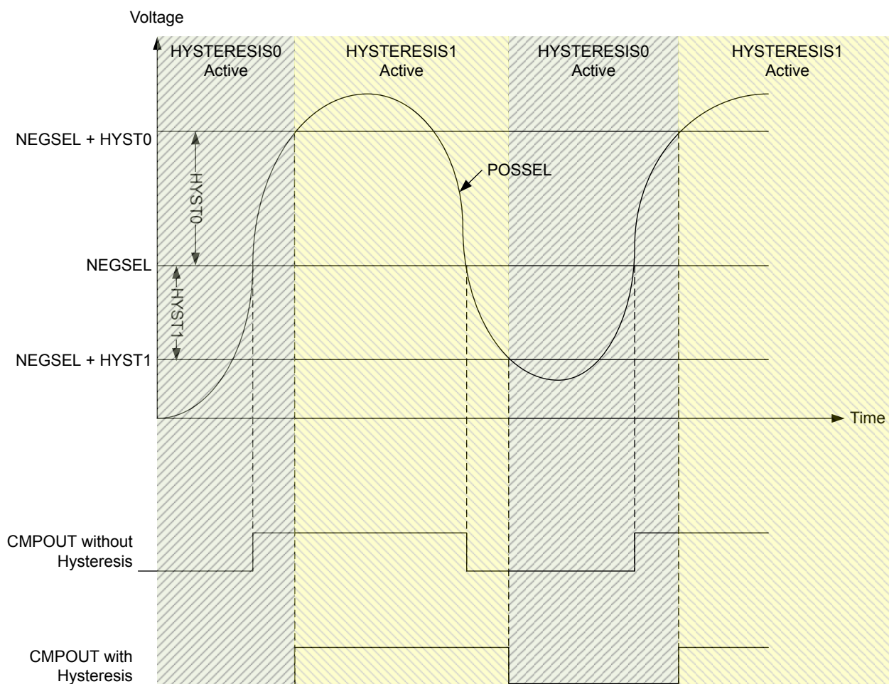
Figure 25.3. Hysteresis
