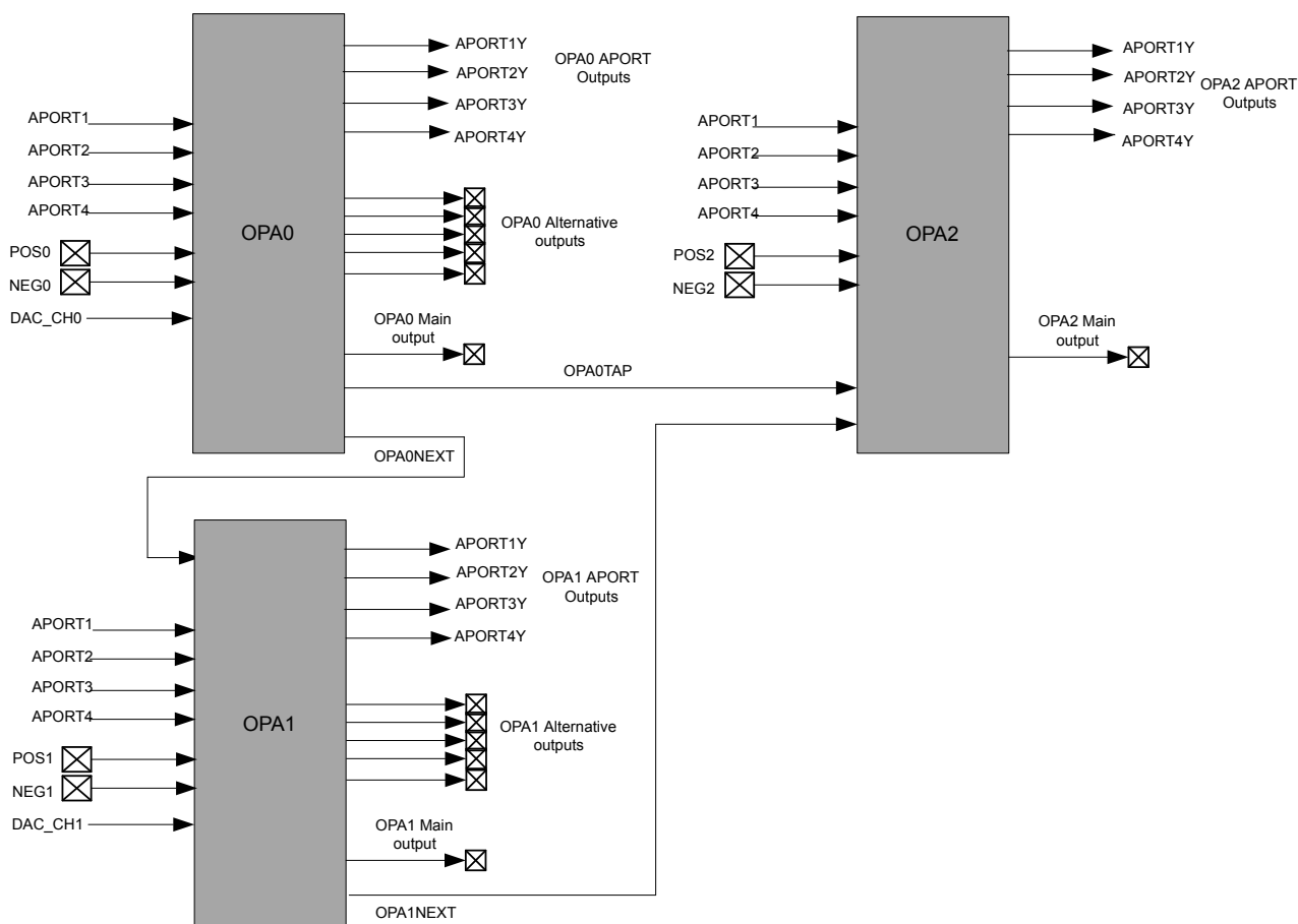
Figure 24.1. OPAMP System Overview
