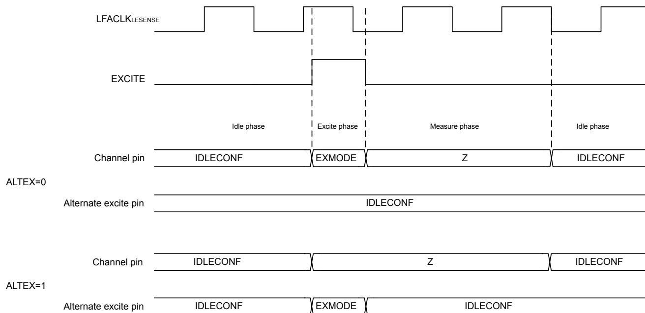
Figure 28.6. Pin Sequencing
