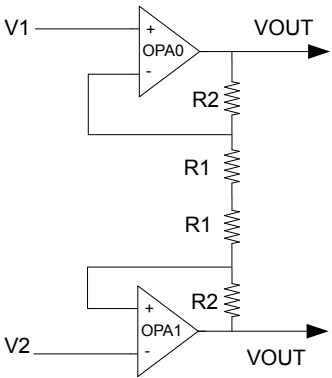
Figure 24.11. Instrumentation Amplifier Overview
