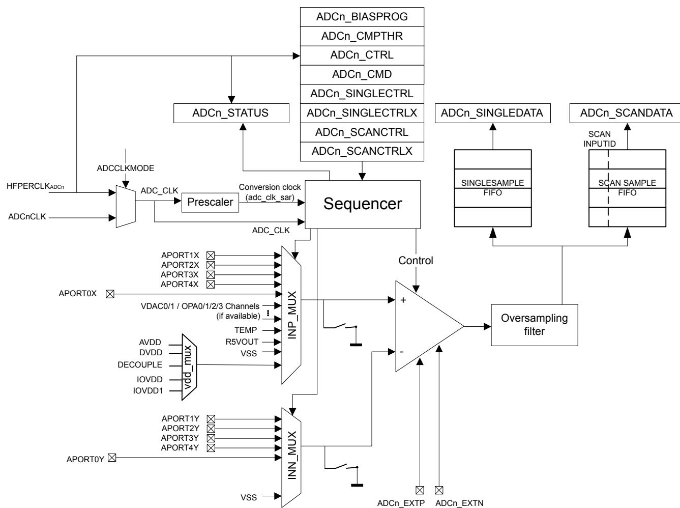
Figure 26.1. ADC Overview
