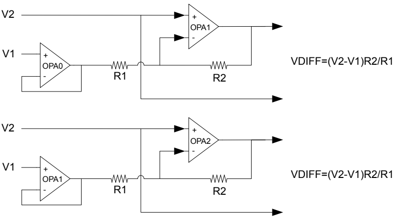
Figure 24.9. Two Op-amp Differential Amplifier Overview
