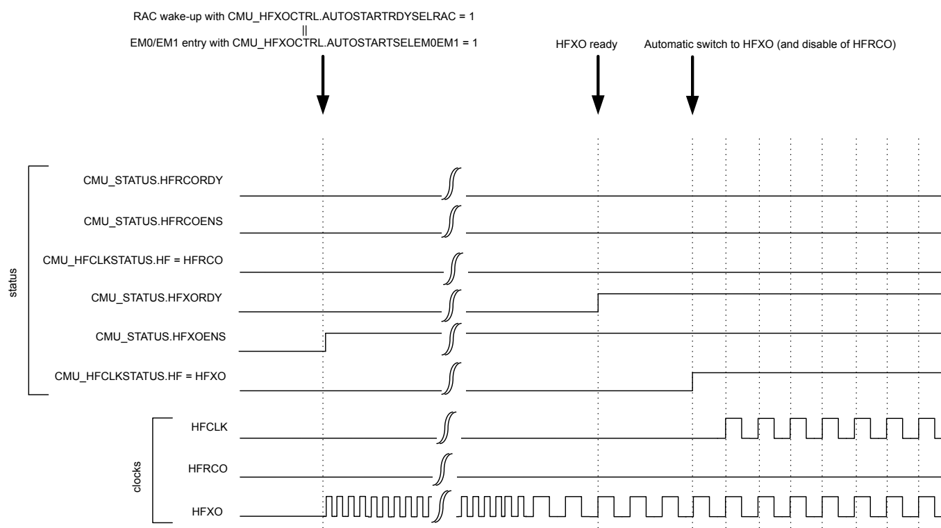
Figure 11.8. CMU Automatic Startup and Selection of HFXO
