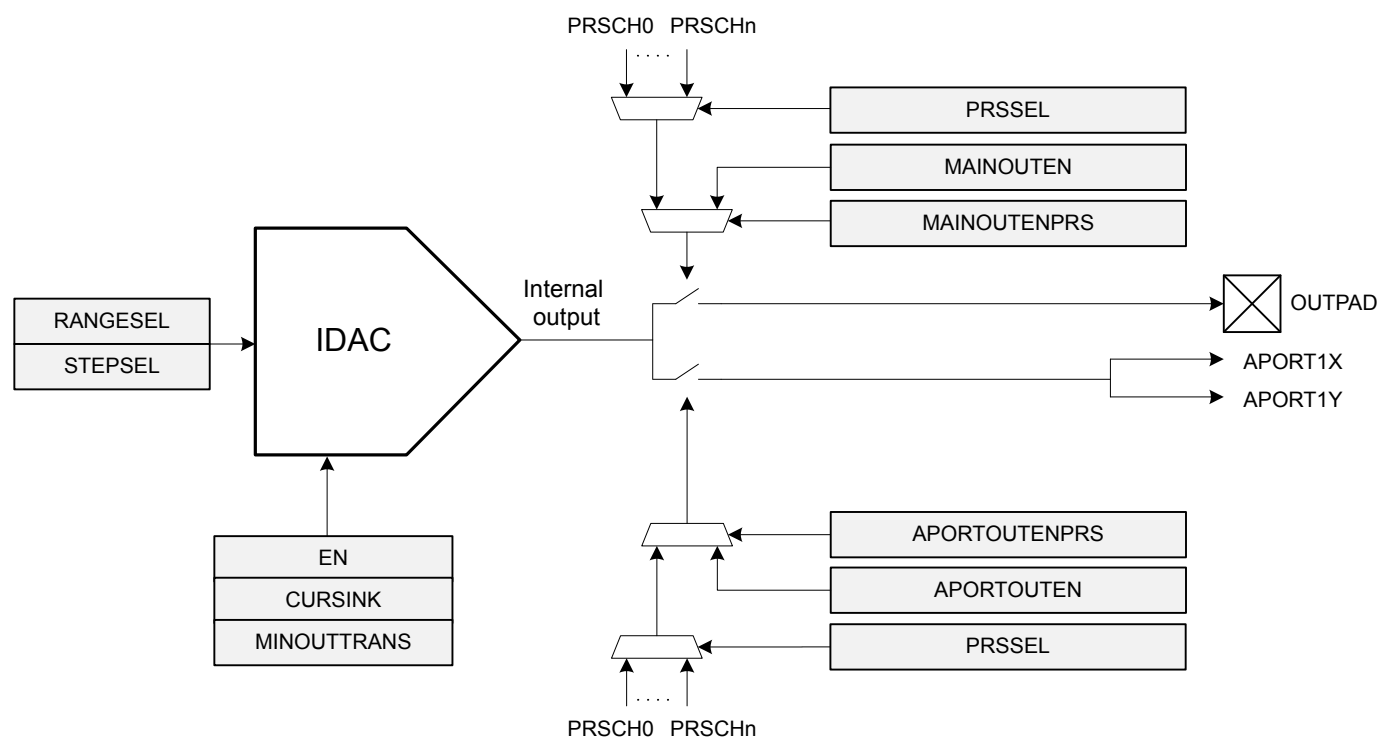
Figure 27.1. IDAC Overview
