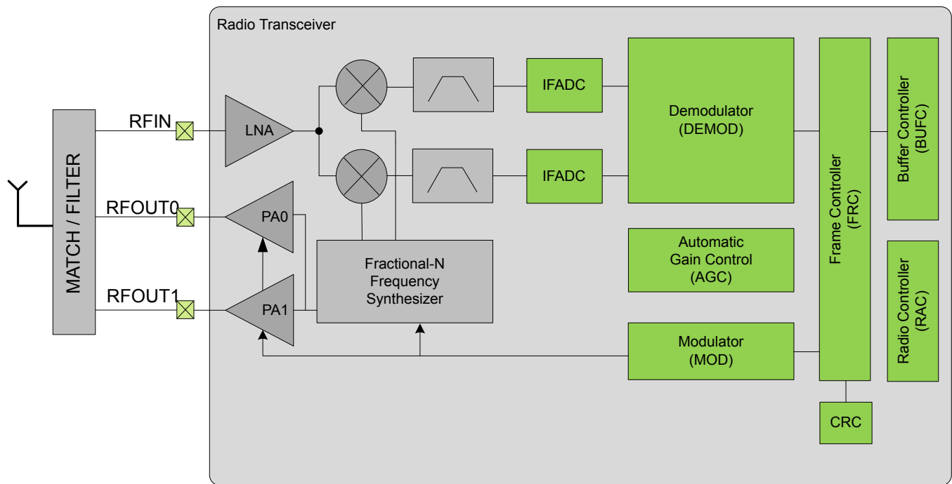
Figure 5.1. Radio Overview
