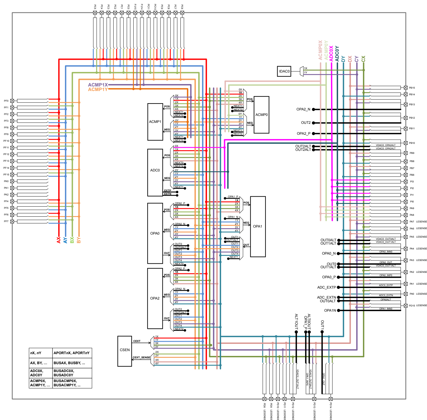
Figure 33.3. Detailed APORT Structure
