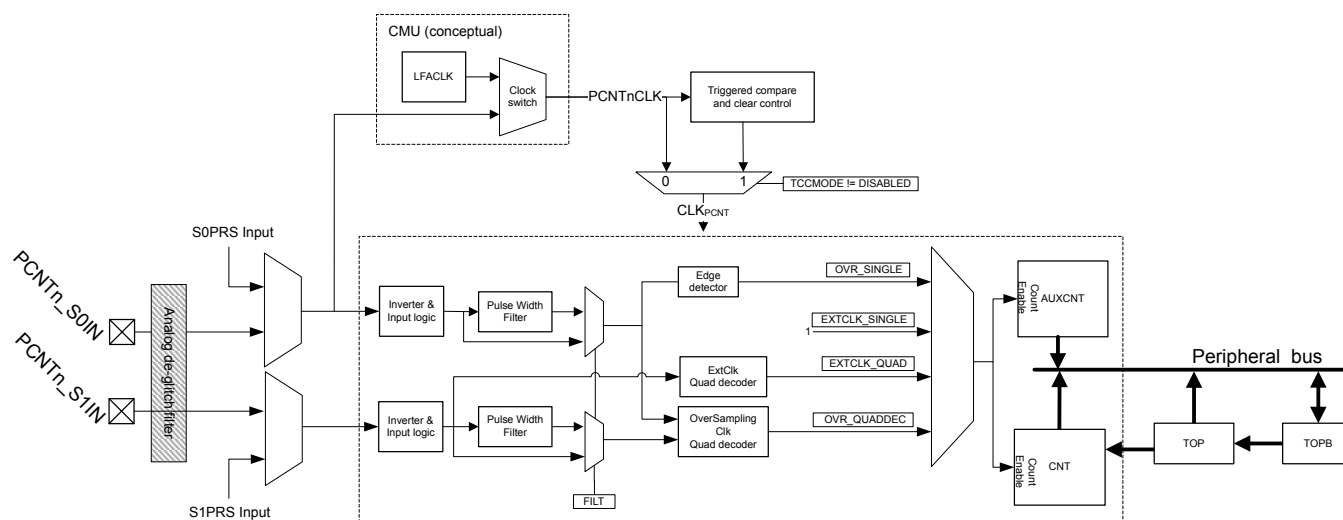
Figure 16.1. PCNT Overview
