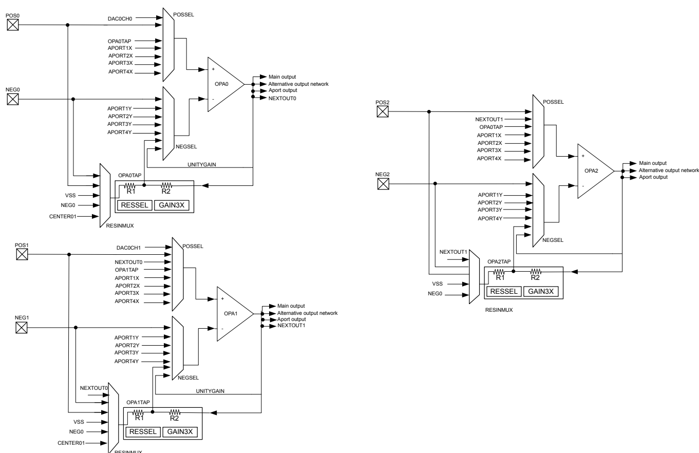
Figure 24.2. OPAMP Overview
