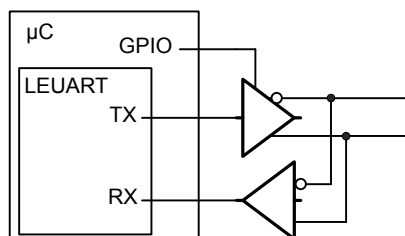
Figure 19.10. LEUART Half Duplex Communication with External Driver
