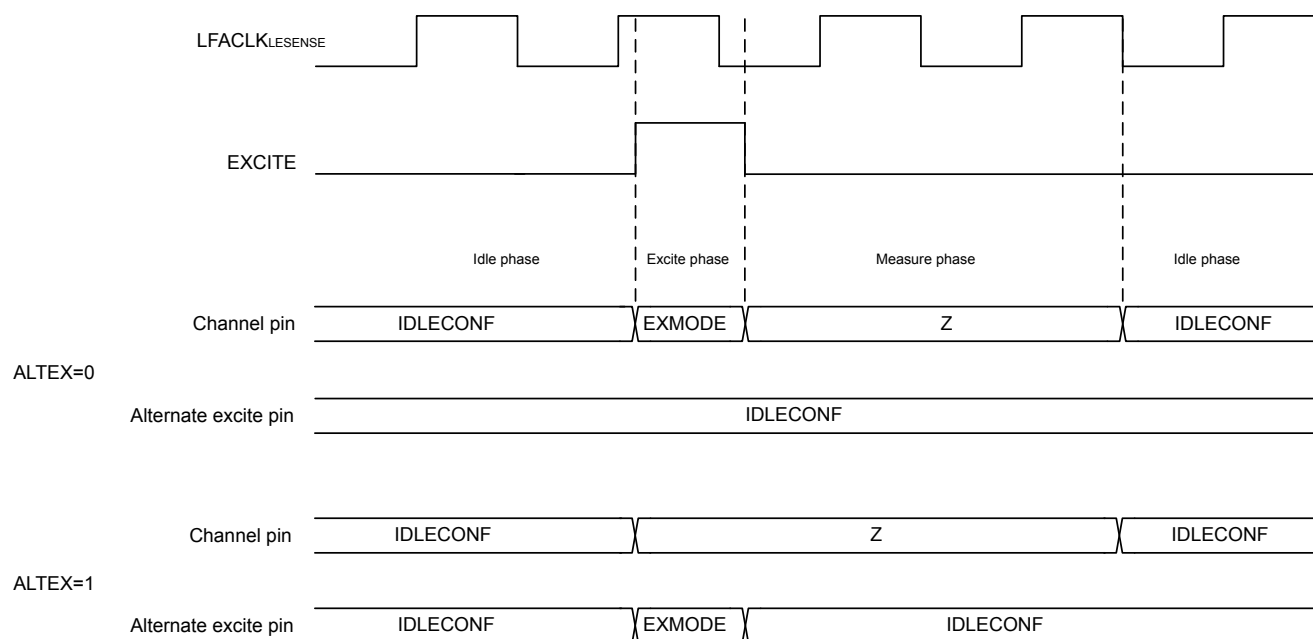
Figure 28.6. Pin Sequencing
