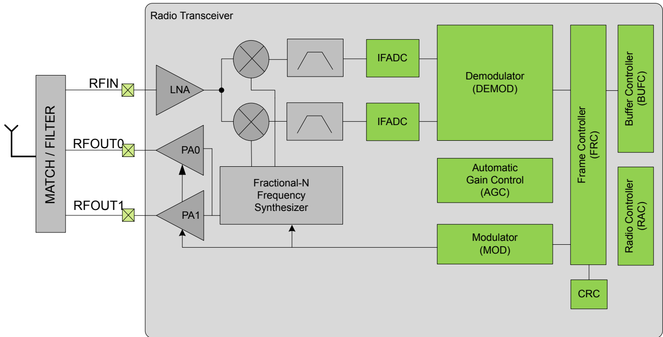
Figure 5.1. Radio Overview
