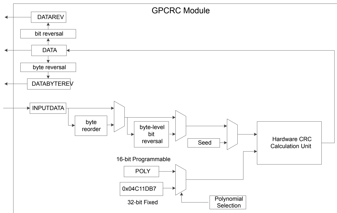
Figure 29.1. GPCRC Overview
