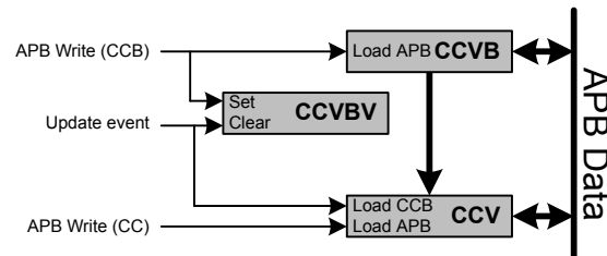
Figure 20.16. TIMER/WTIMER Output Compare/PWM Buffer Functionality Detail
