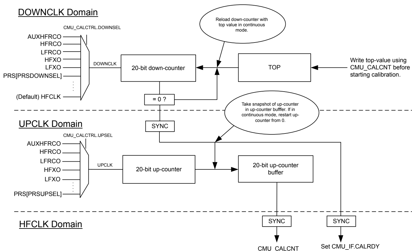
Figure 11.13. HW-support for RC Oscillator Calibration
