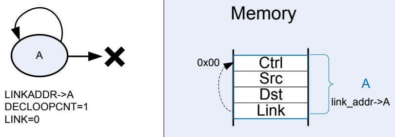
Figure 8.6. Single Descriptor Looped Transfer
