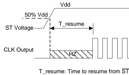
Figure 5. Standby Resume Timing (ST, \overline{\text{ST}} Mode Only)
