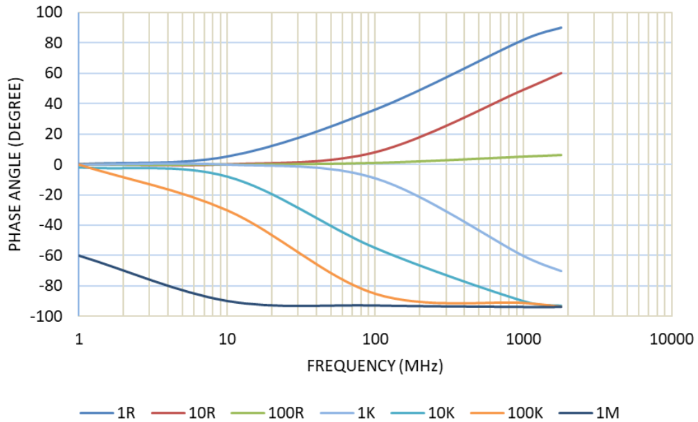
MLFA1 FREQUENCY x PHASE ANGLE
