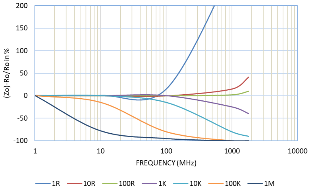
MLFA25 FREQUENCY x IMPEDANCE
