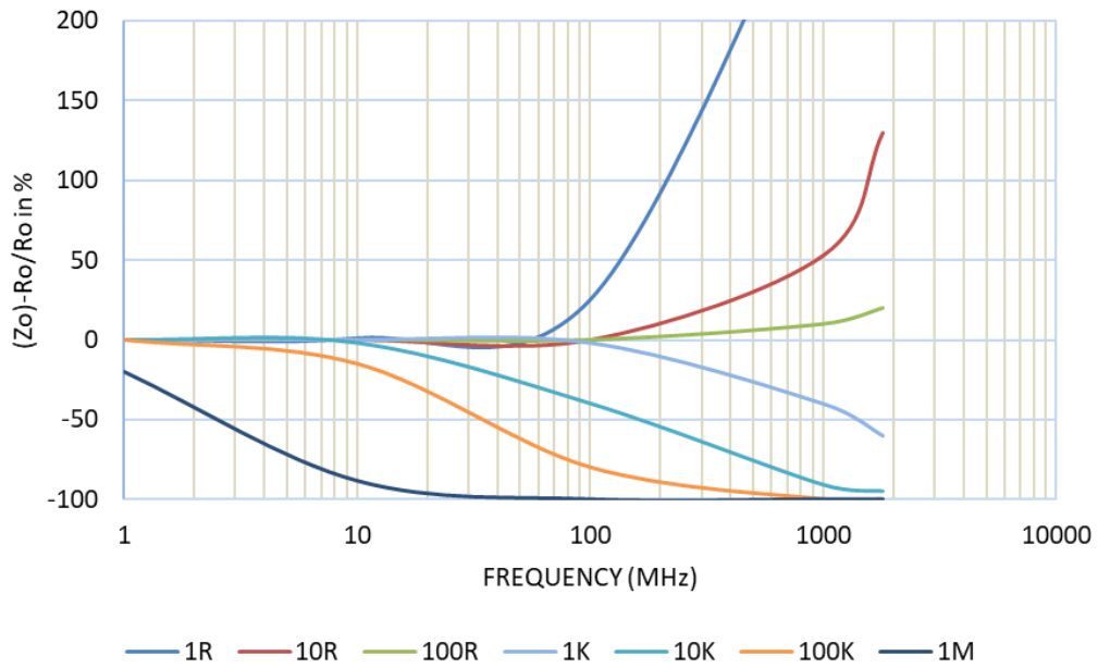
MLFA1 FREQUENCY x IMPEDANCE
