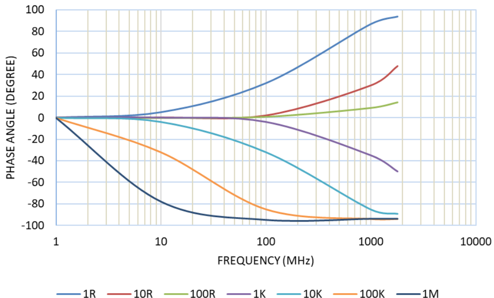
MLFA25 FREQUENCY x PHASE ANGLE
