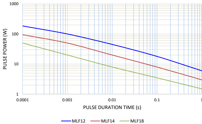
SINGLE PULSE ( R < 10\Omega )
