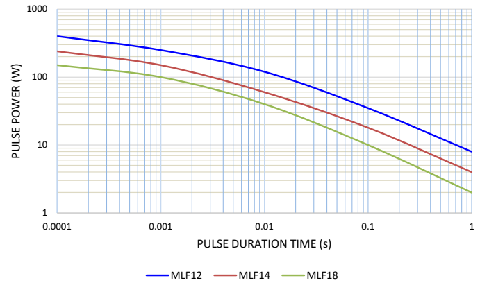
SINGLE PULSE ( R \geq 10\Omega )
