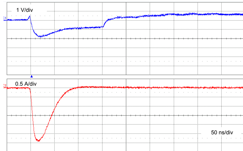
Figure 9. ISO7637-3 pulse 3a response (V S = -150 V)
