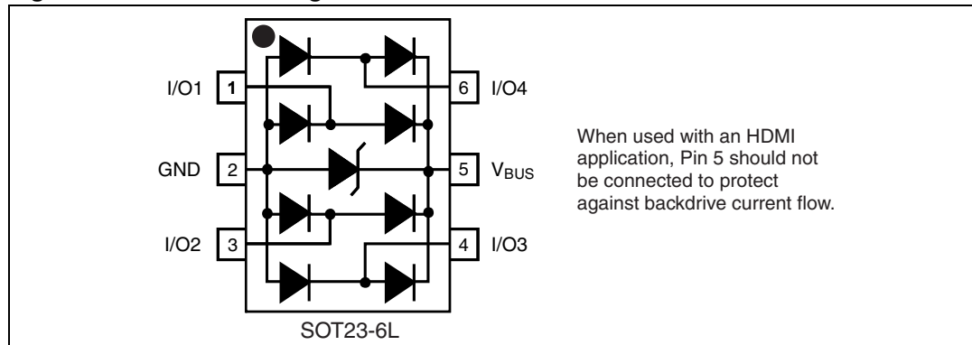
Figure 1. Functional diagrams
