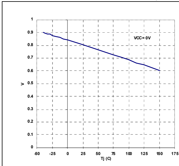
Figure 9. UVLO saturation vs. T_J
