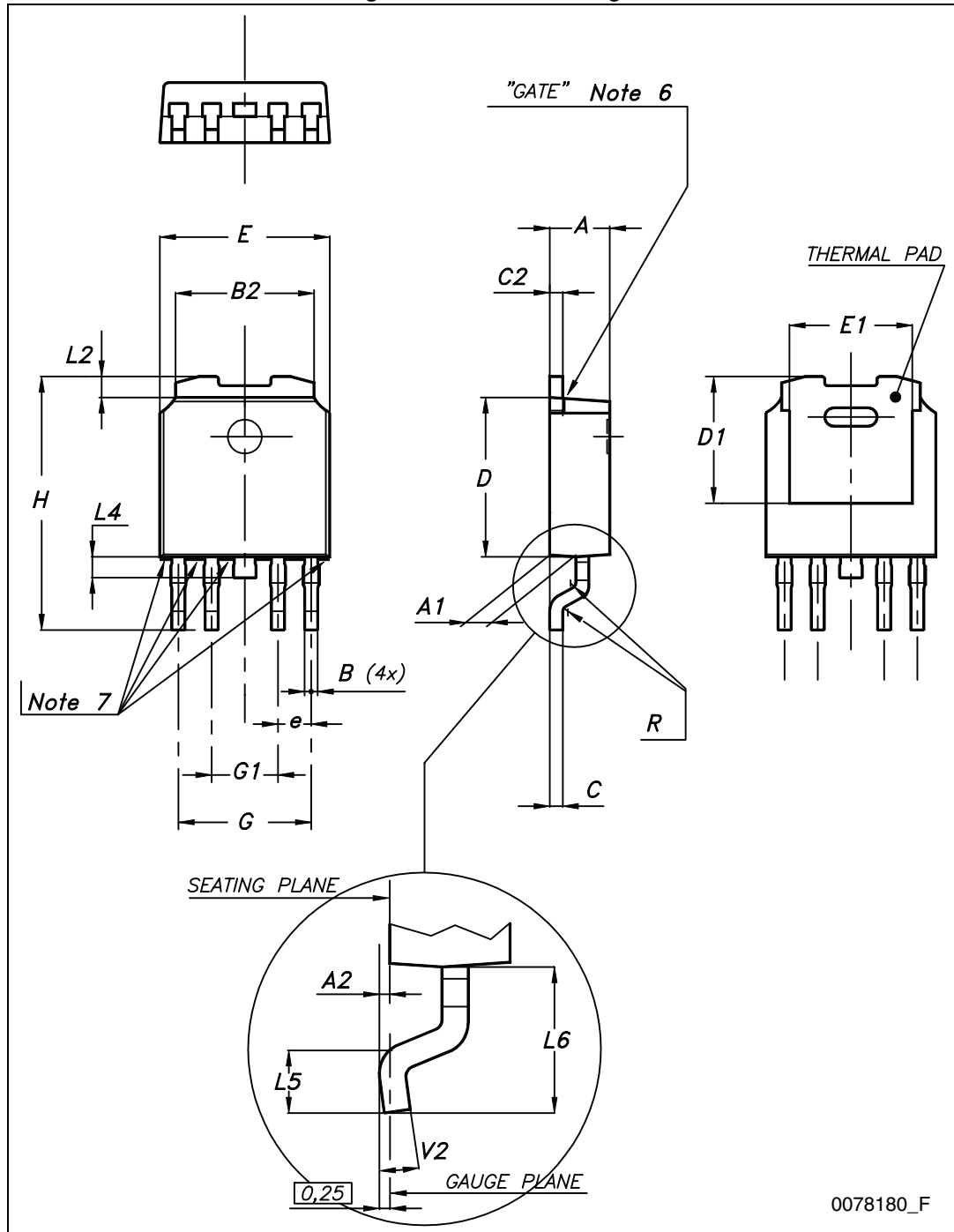
Figure 20. PPAK drawing
