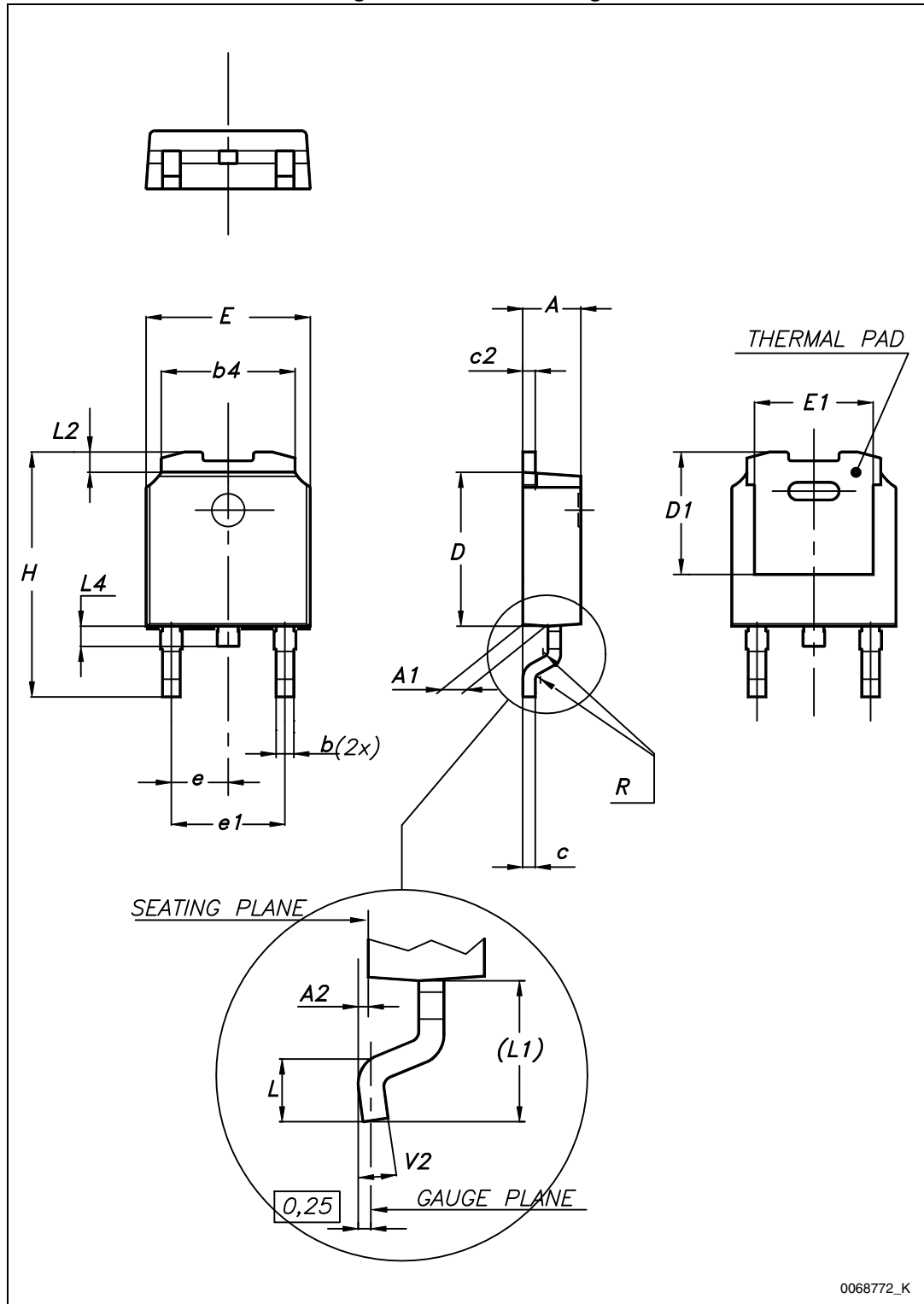
Figure 21. DPAK drawing
