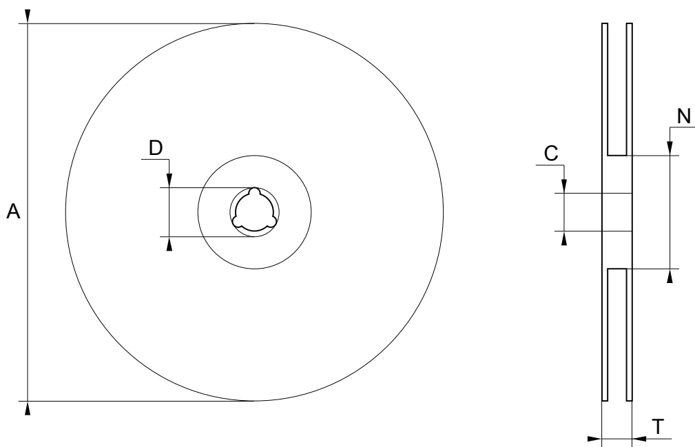
Figure 56. Reel outline
