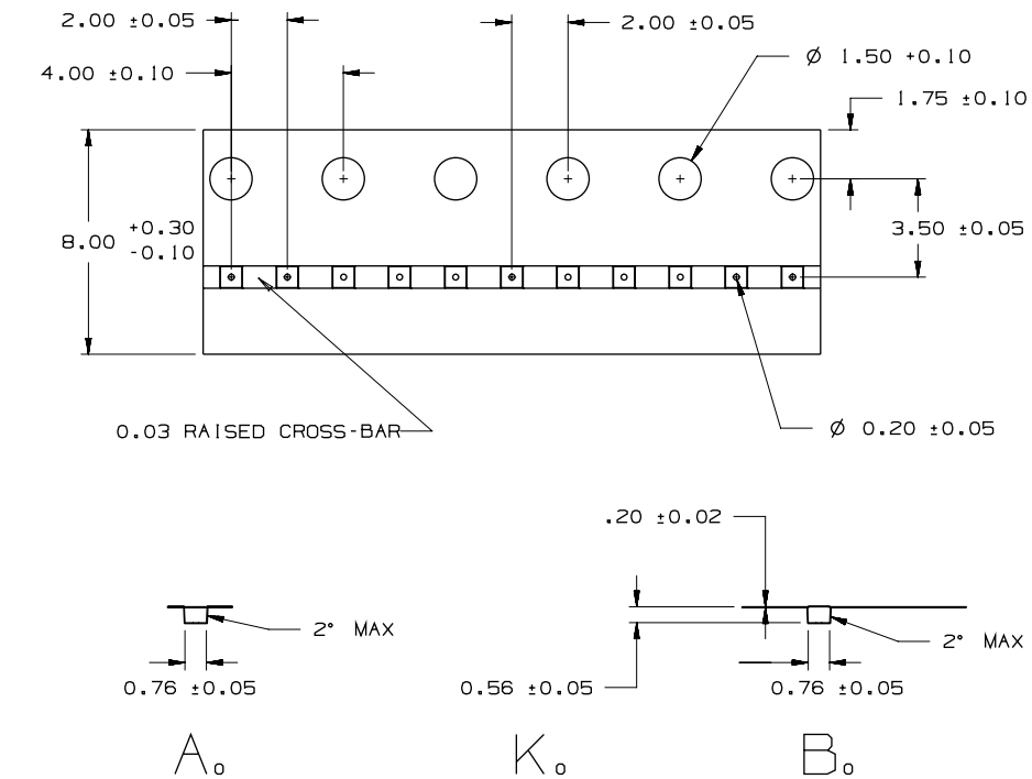
Figure 52. Flip-chip 4 tape for LD39130SJ30R
