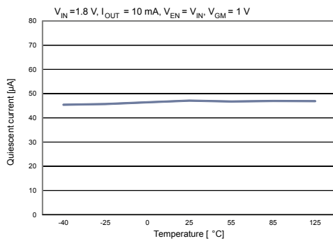
Figure 15. Quiescent current vs. temperature ( I_{OUT} = 10 mA, normal mode)
