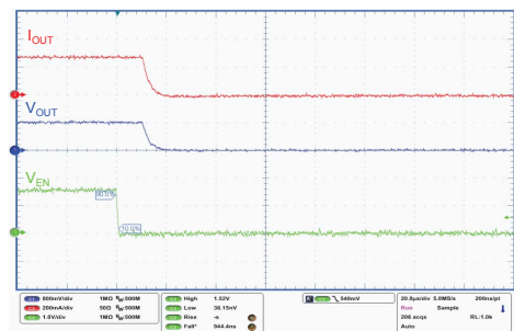
Figure 40. Turn-off time
