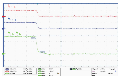
Figure 40. Turn-off time
