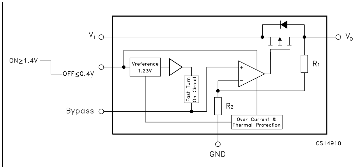
Figure 1. Schematic diagram
