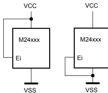
Figure 5. Chip enable inputs connection
