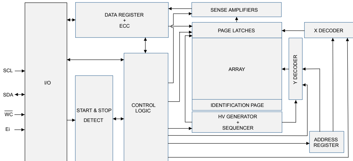
Figure 6. Block diagram
