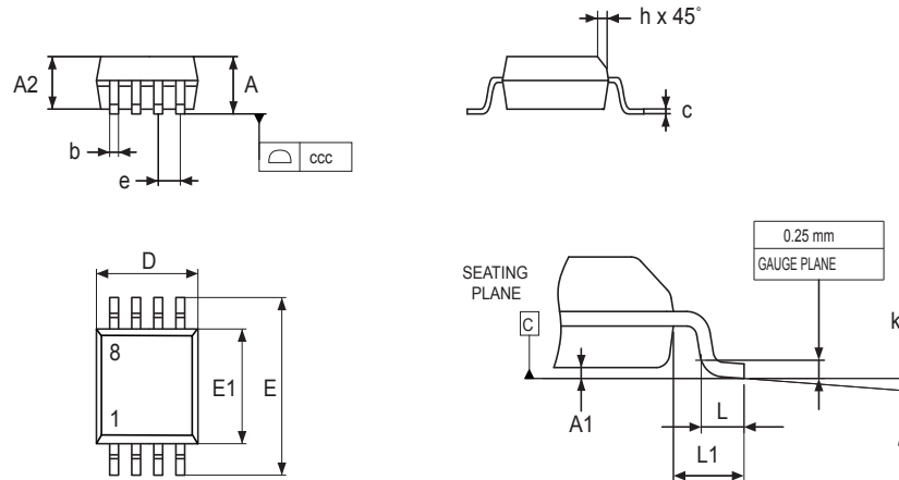
Figure 22. SO8N - Outline
