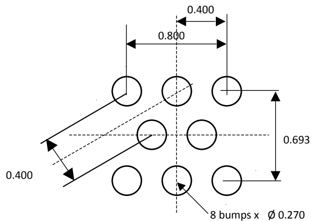
Figure 25. WLCSP8 - Footprint example
