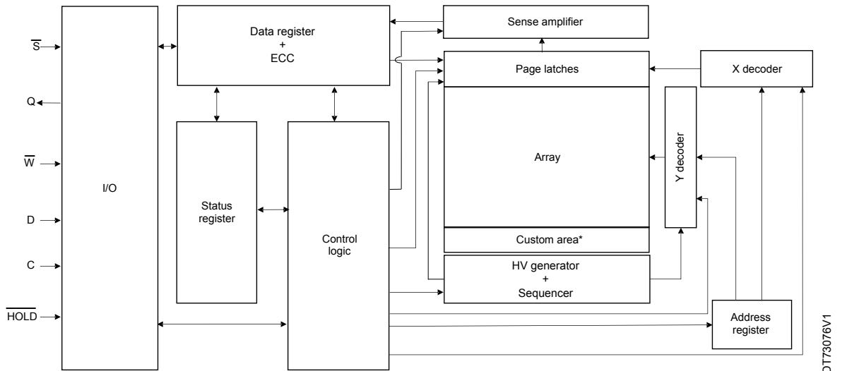
Figure 3. Block diagram
