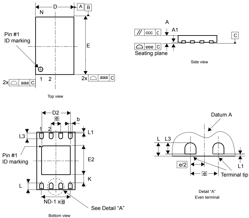
Figure 26. UFDFPN8 - Outline
