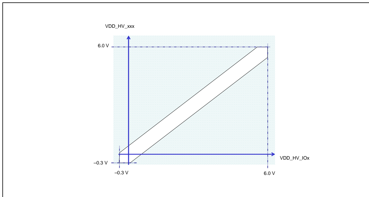
Figure 6. Power supplies constraints ( -0.3 V \leq V_{DD\_HV\_IOx} \leq 6.0 V)
