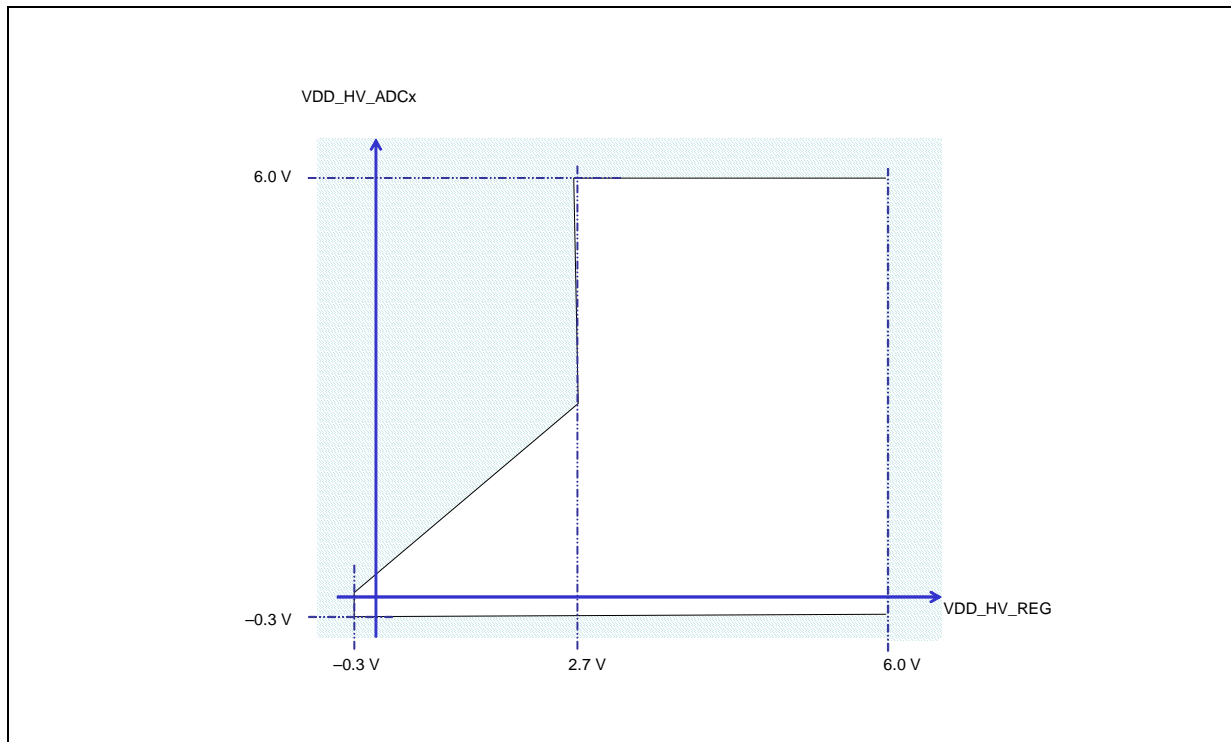
Figure 7. Independent ADC supply ( -0.3 \text{ V} \leq V_{\text{DD\_HV\_REG}} \leq 6.0 \text{ V} )
