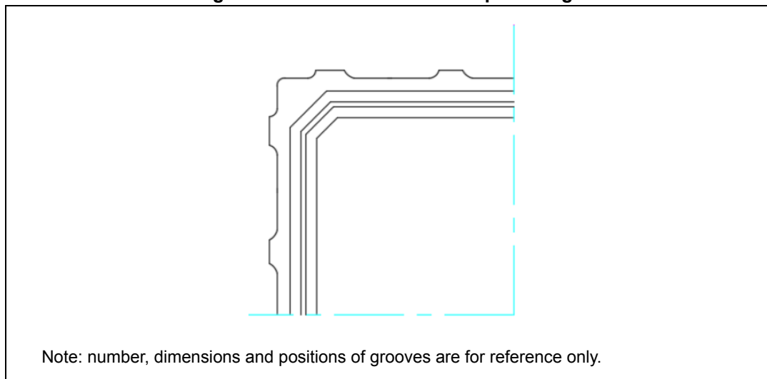
Figure 53. eLQFP176 leadframe pad design
