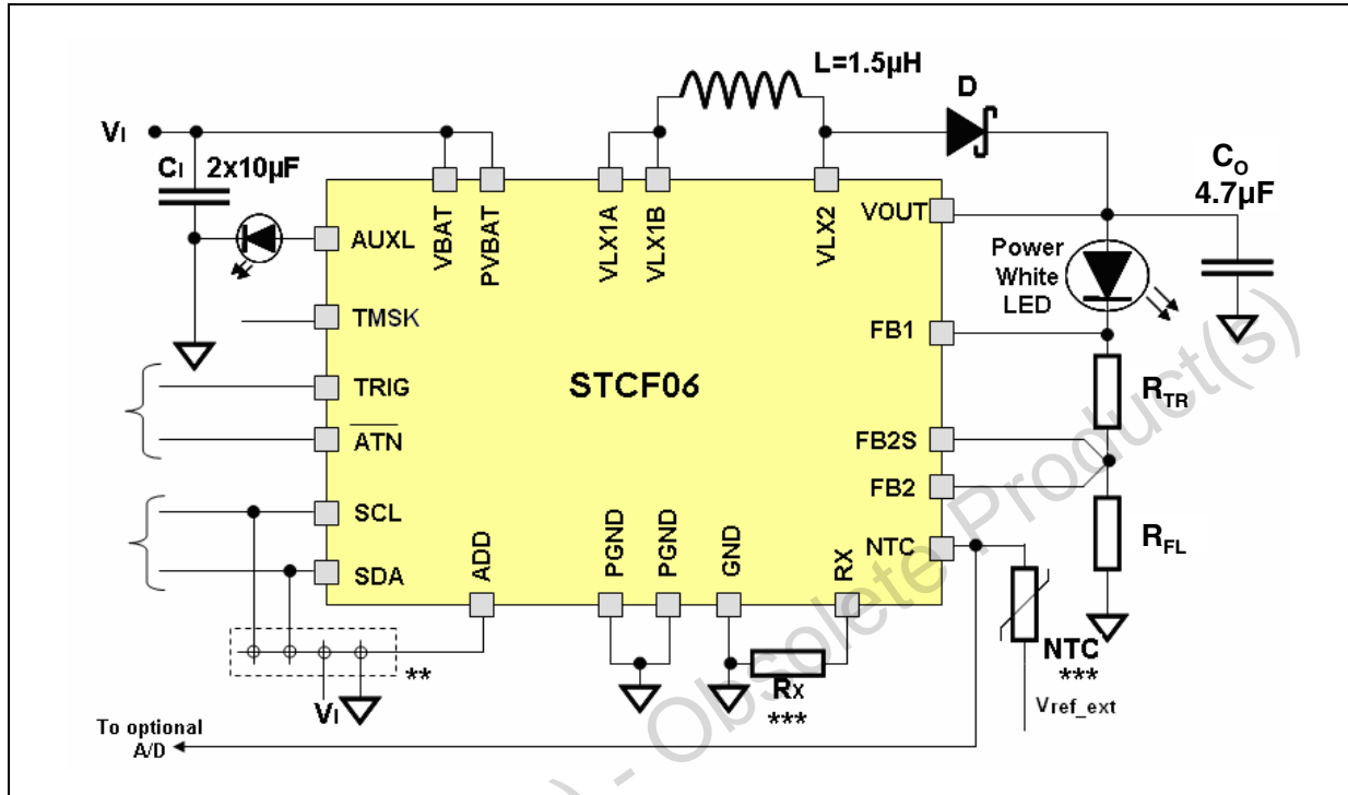
Figure 3. Application schematic
