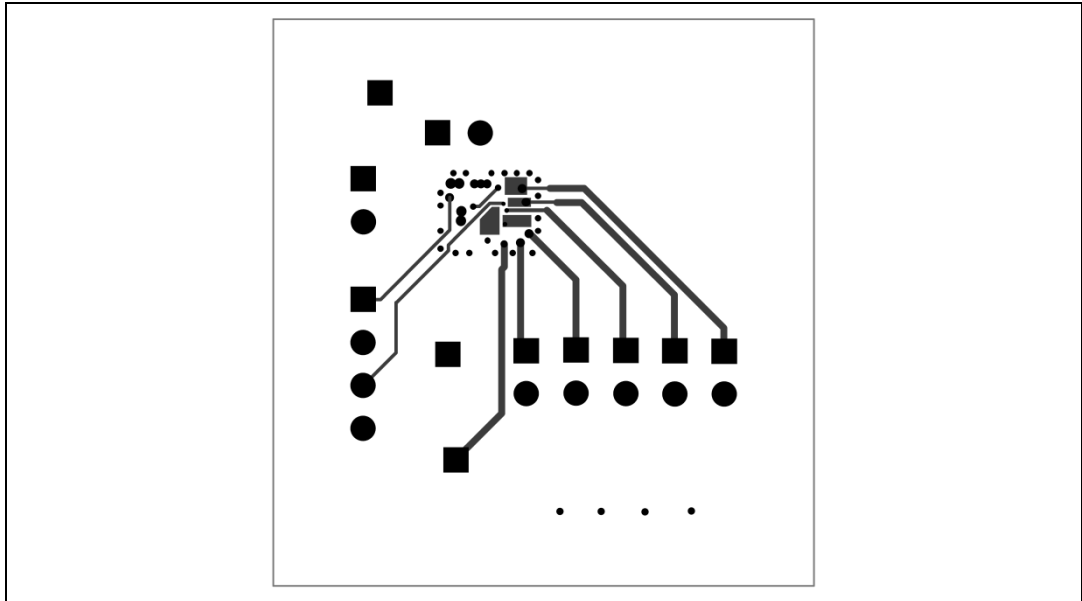
Figure 22. Mid layer 2
