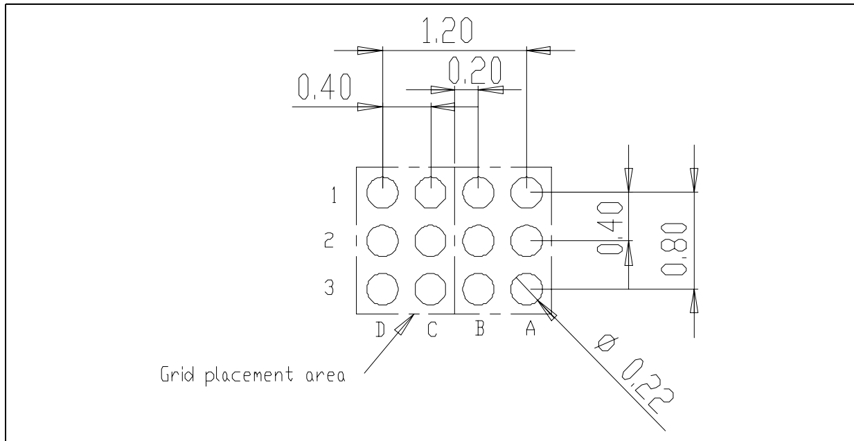
Figure 26. Footprint recommended data (mm.)
