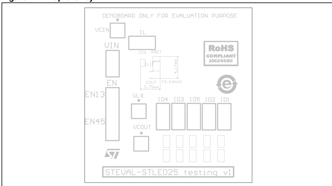
Figure 24. Top overlay
