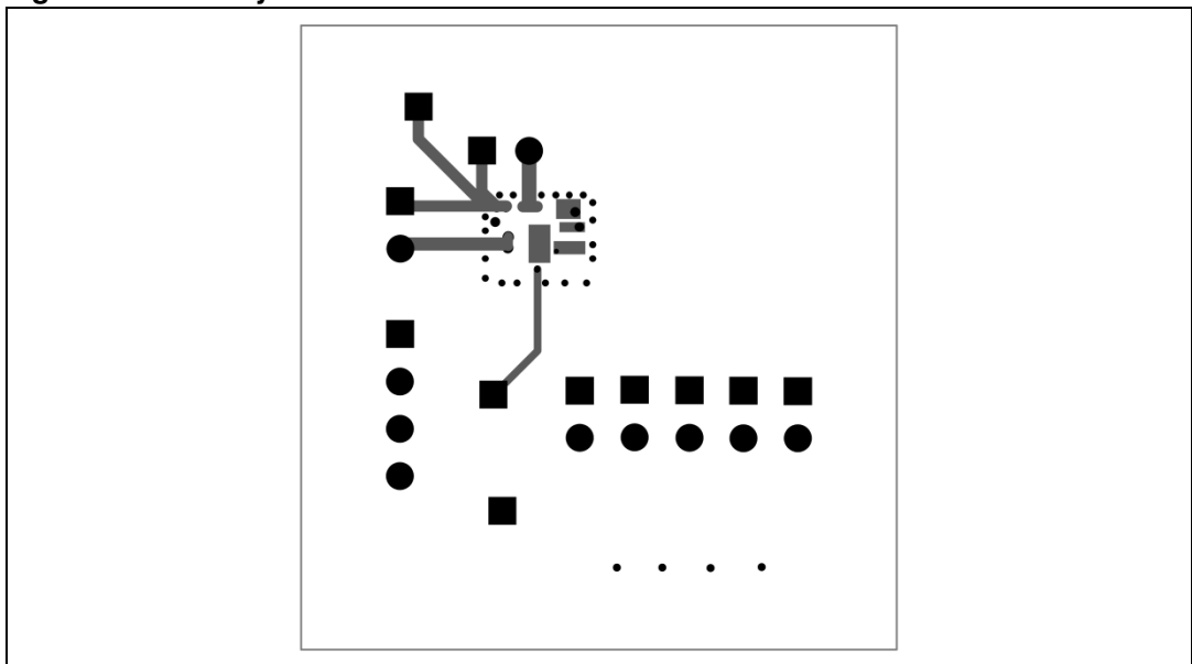
Figure 22. Mid layer 2
