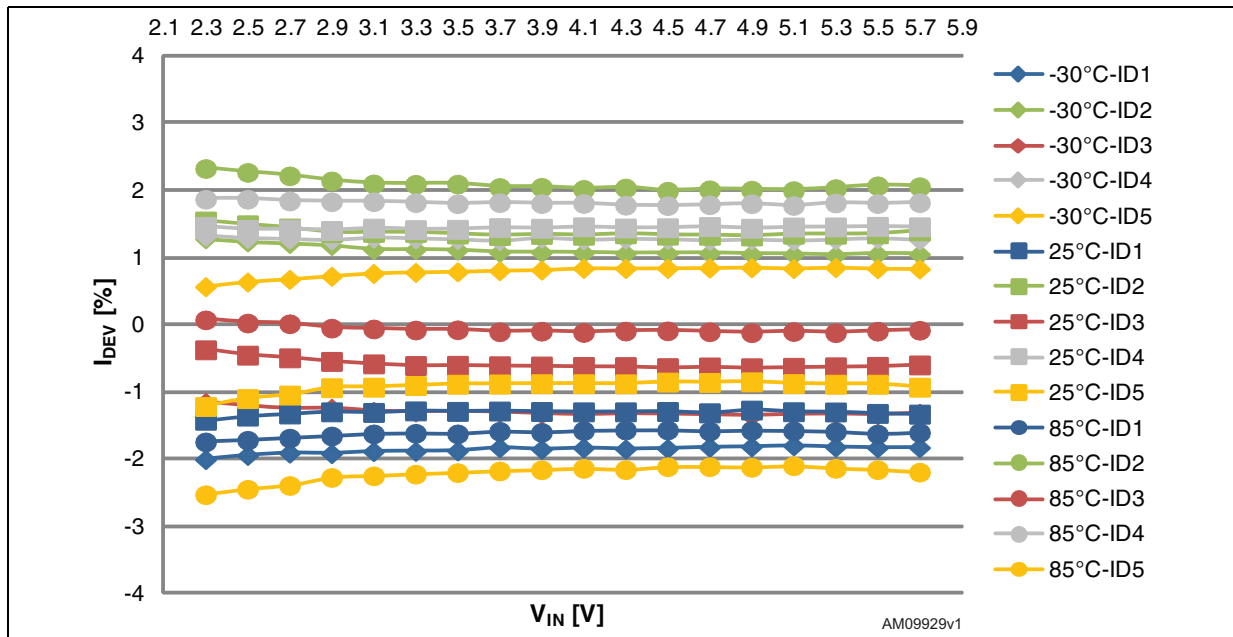
Figure 11. Current matching - set string current to 20 mA
