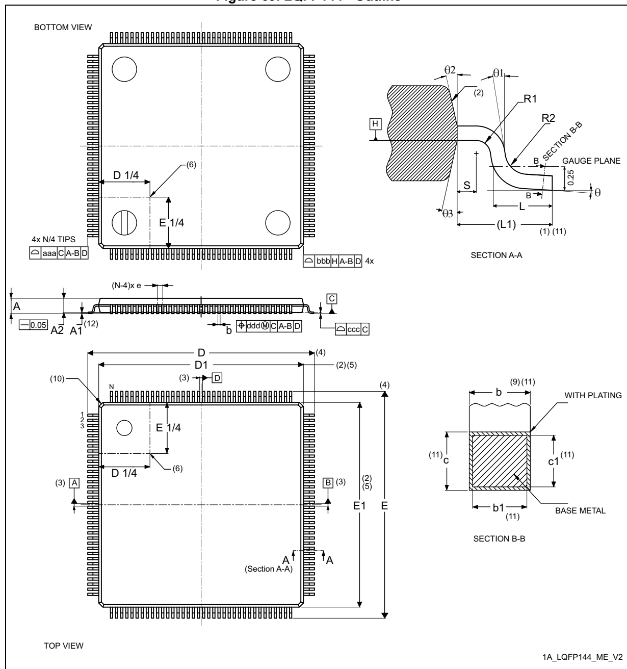
Figure 69. LQFP144 - Outline (15)
