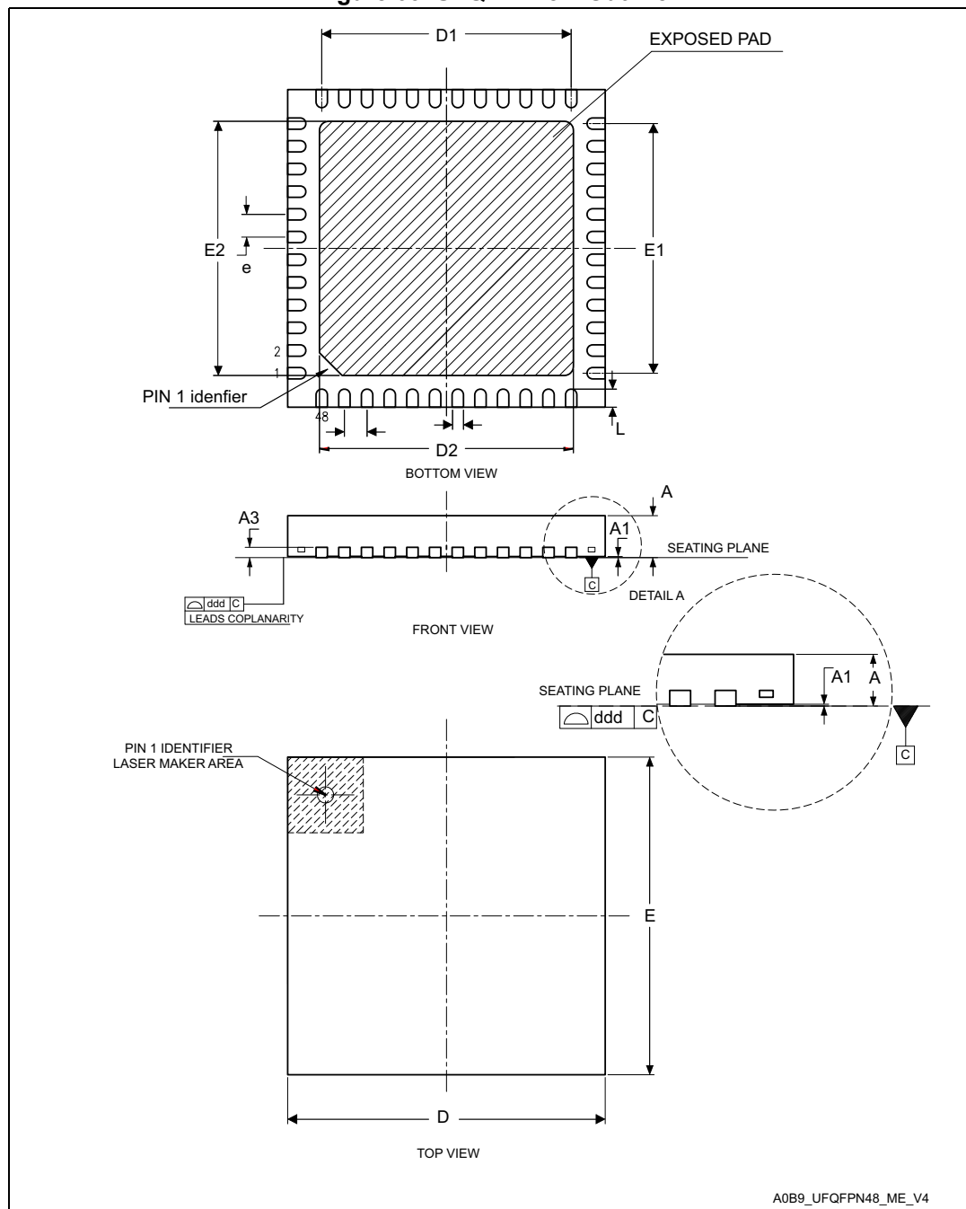
Figure 63. UFQFPN48 – Outline
