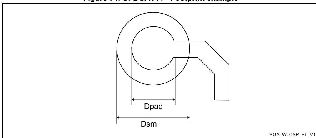
Figure 74. UFBGA144 - Footprint example
