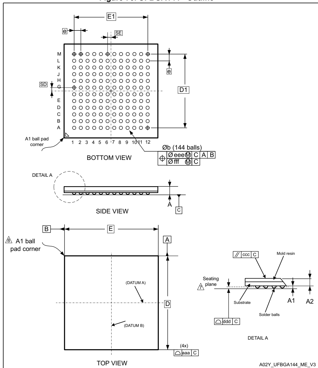
Figure 73. UFBGA144 - Outline (13)
