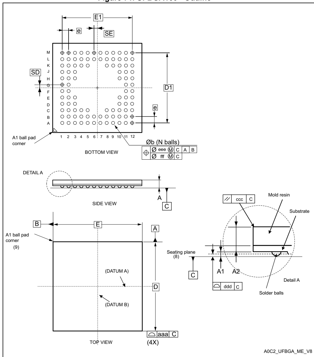
Figure 71. UFBGA100 - Outline (13)
