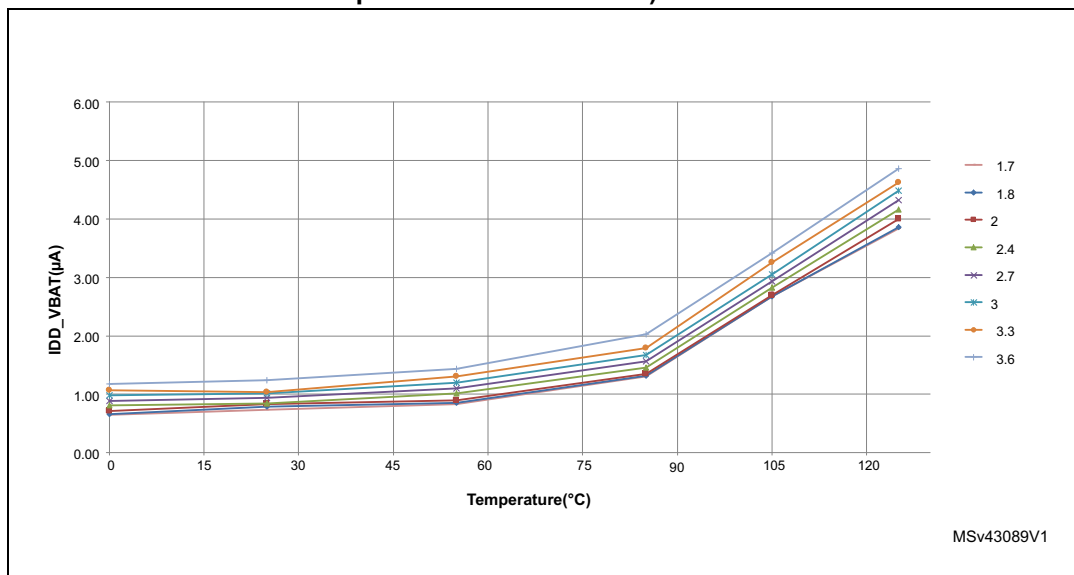
Figure 25. Typical V_{BAT} current consumption (LSE and RTC ON/LSE oscillator “high drive” mode selection)
