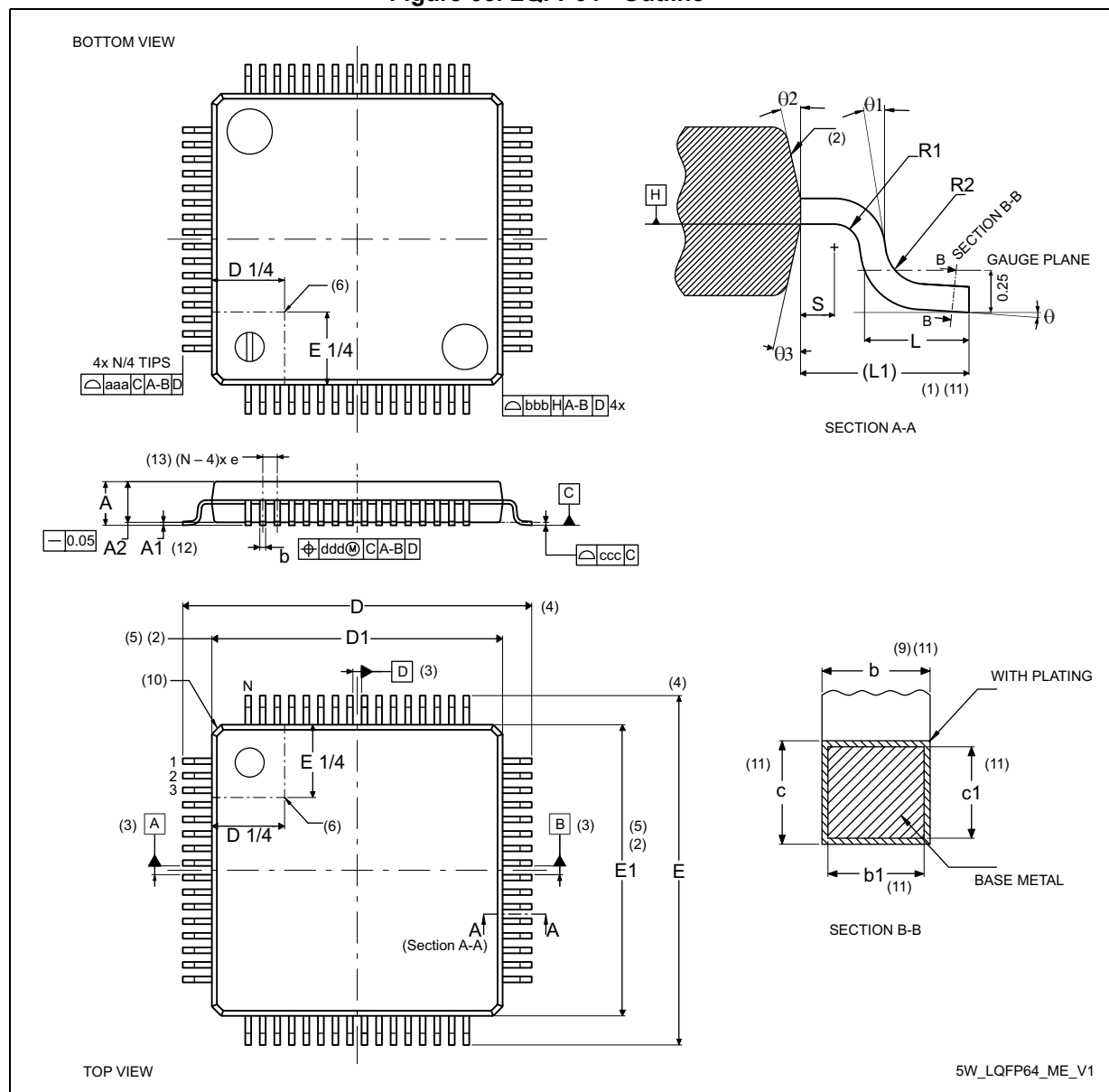
Figure 65. LQFP64 - Outline (15)
