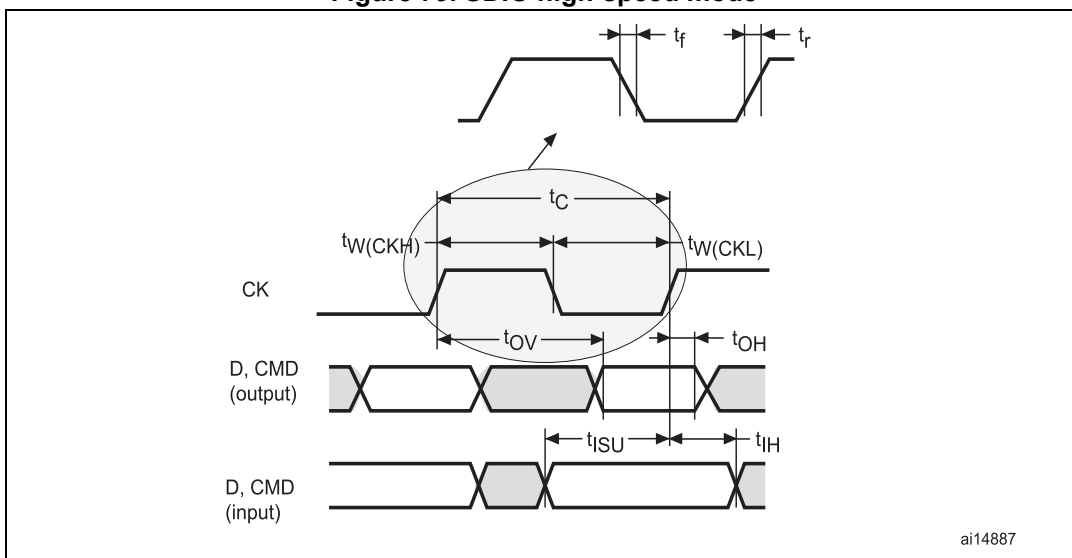
Figure 79. SDIO high-speed mode
