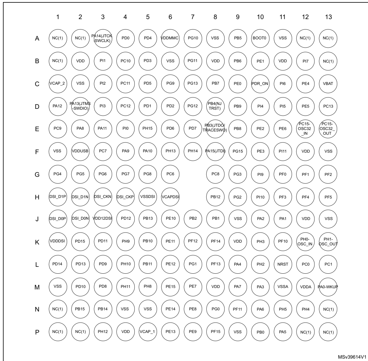
Figure 17. STM32F779Ax/STM32F778Ax WLCSP180 ballout
