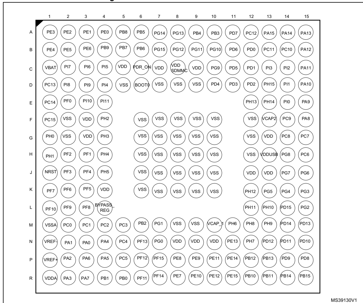
Figure 16. STM32F77xxx UFBGA176 ballout
