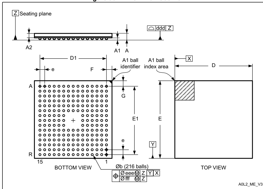
Figure 96. TFBGA216 - Outline
