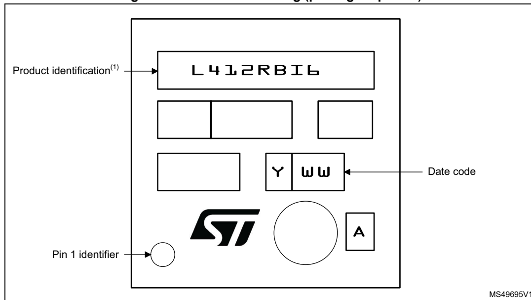
Figure 47. UFBGA64 marking (package top view)
