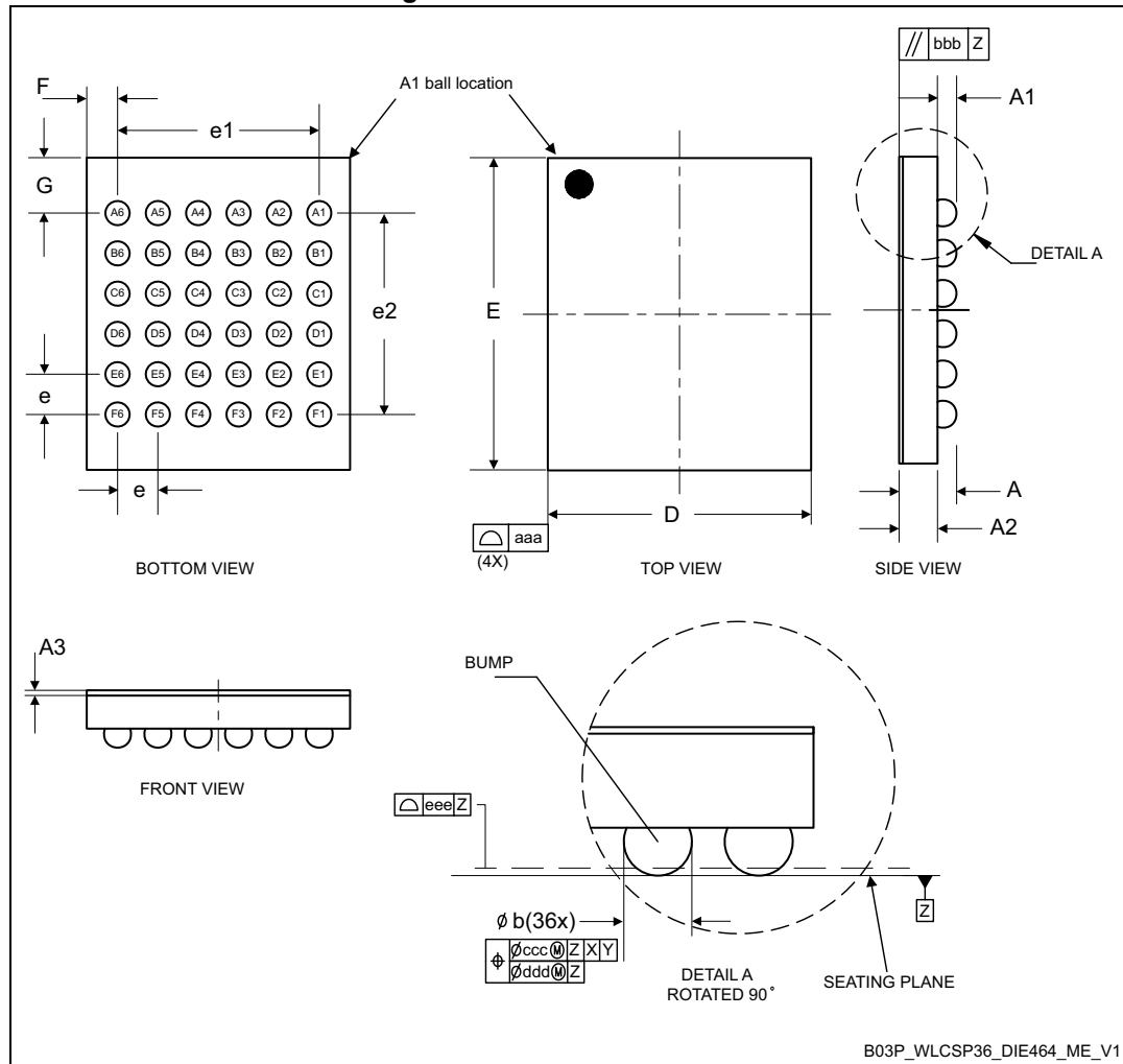
Figure 47. WLCSP36 - Outline
