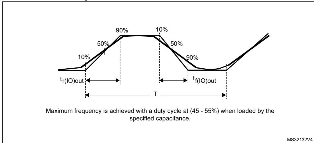
Figure 26. I/O AC characteristics definition (1)
