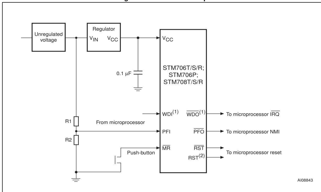
Figure 9. Hardware hookup
