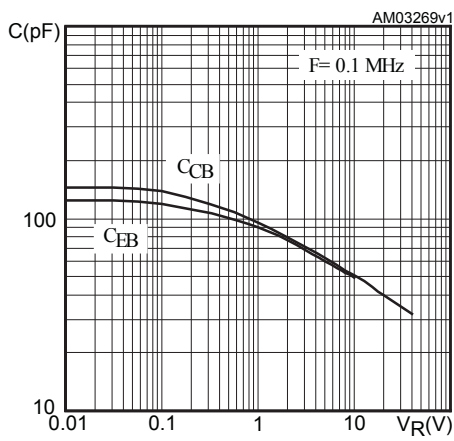
Figure 15. Capacitance characteristics (NPN)
