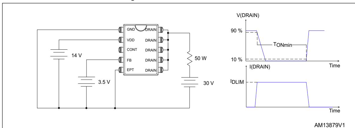
Figure 4. Minimum turn-on time test circuit
