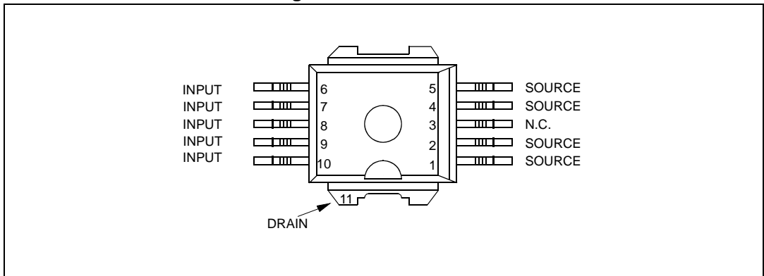
Figure 2. Pin connection
