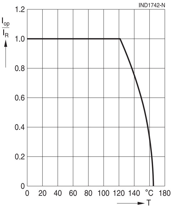
Current derating I_{\text{op}}/I_{\text{R}} versus ambient temperature T_{\text{A}}
