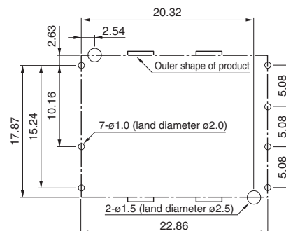
Recommended measurements for mounting board
