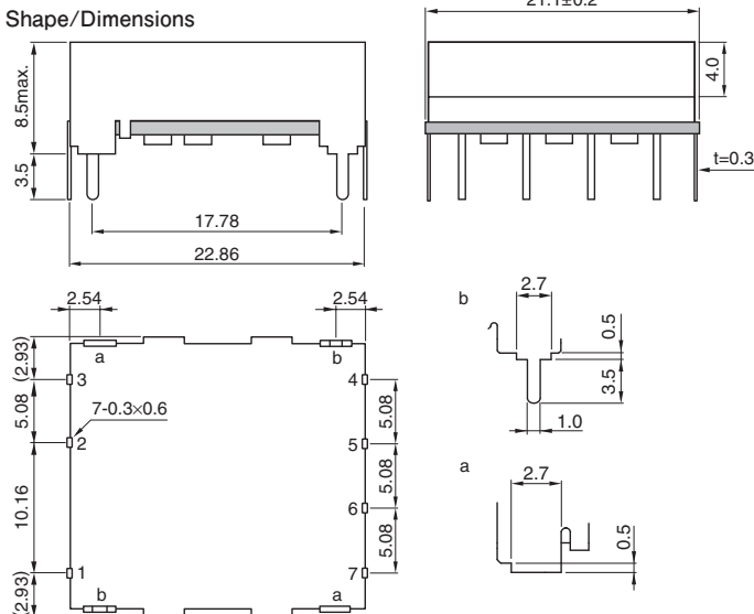
Shape/Dimensions
