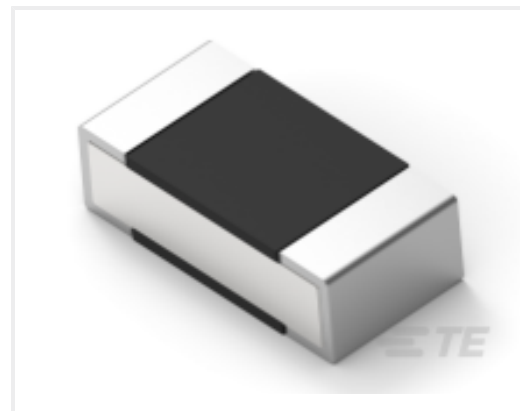
TE Part #2176304-1 RP 1E 0.1W 10R 0.1% 25PPM 5K RL
