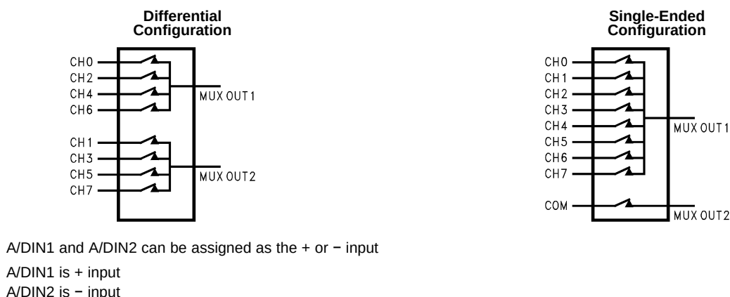
Figure 68. MUXOUT connections for multiplexer option
