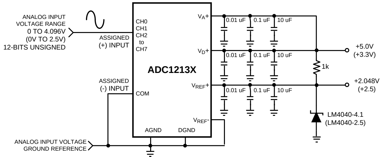
Figure 69. Single-Ended Biasing
