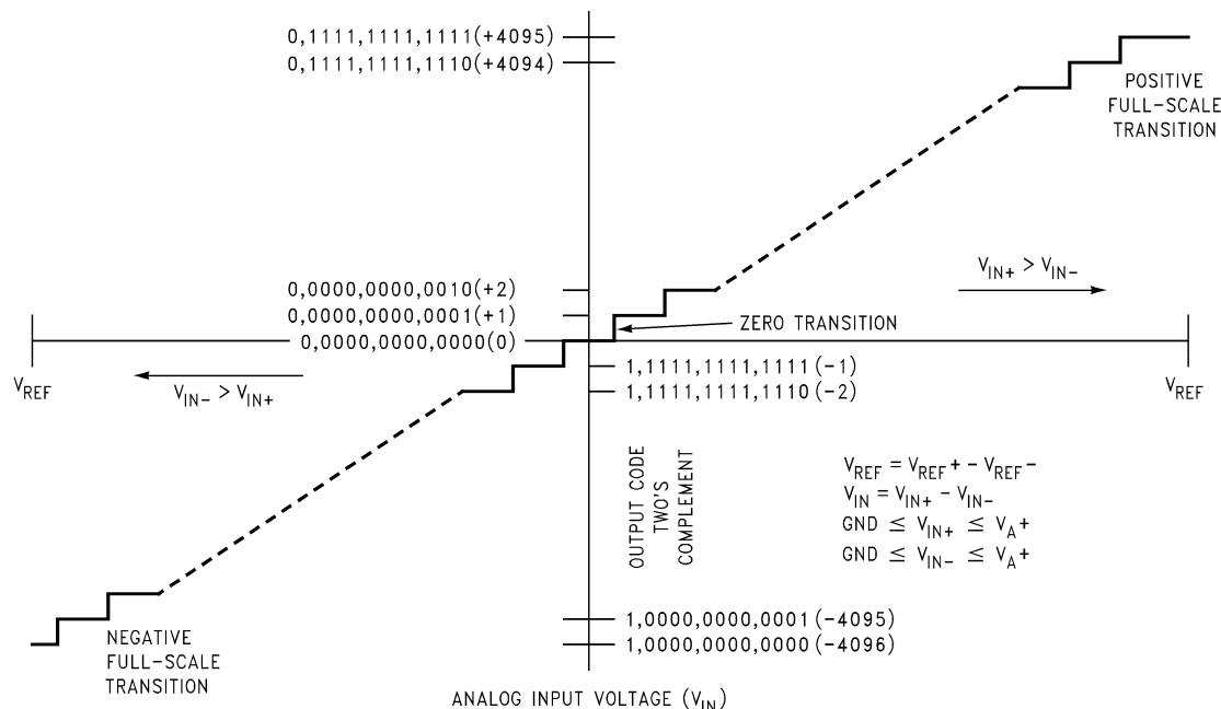
Figure 4. Transfer Characteristic
