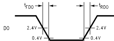
Figure 49. DO Falling and Rising Edge
