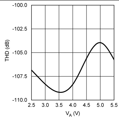
Figure 18. THD vs. V_A
