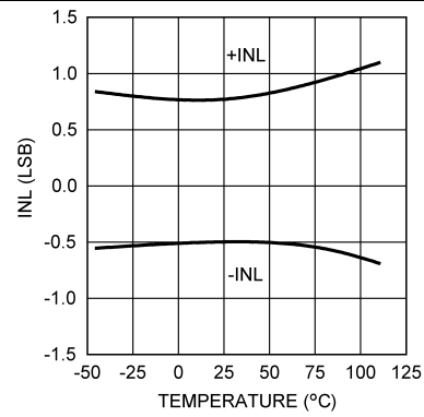
Figure 16. INL vs. Temperature
