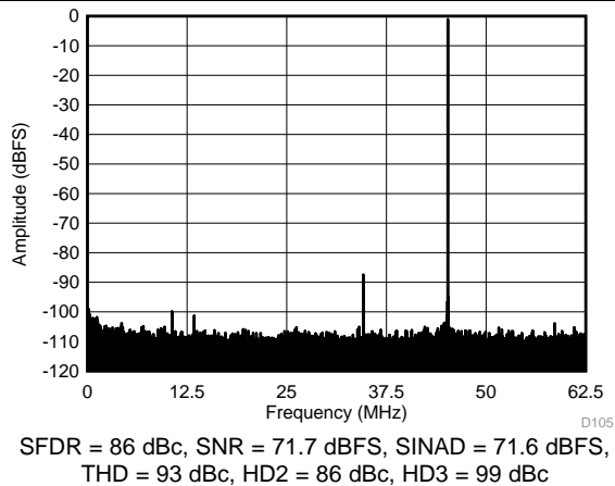
Figure 104. FFT for 170-MHz Input Signal (Dither On)
