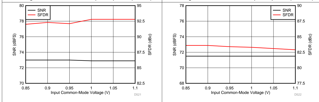
Figure 54. Performance vs Input Common-Mode Voltage (30 MHz)
