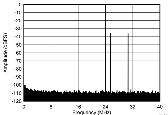
f_{IN1} = 185 \text{ MHz} , f_{IN2} = 190 \text{ MHz} , IMD3 = 106 dBFS, each tone at -36 dBFS
