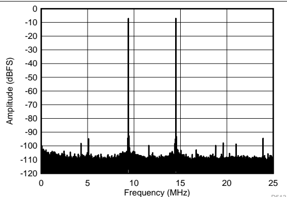
f_{IN1} = 185 \text{ MHz} , f_{IN2} = 190 \text{ MHz} , IMD3 = 93 dBFS, each tone at -7 dBFS
