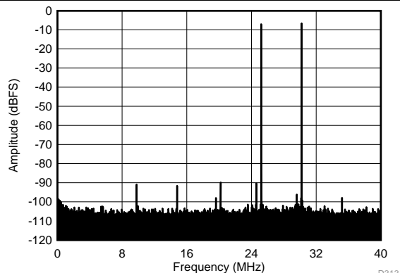
f_{IN1} = 185 \text{ MHz} , f_{IN2} = 190 \text{ MHz} , IMD3 = 90 dBFS, each tone at -7 dBFS
