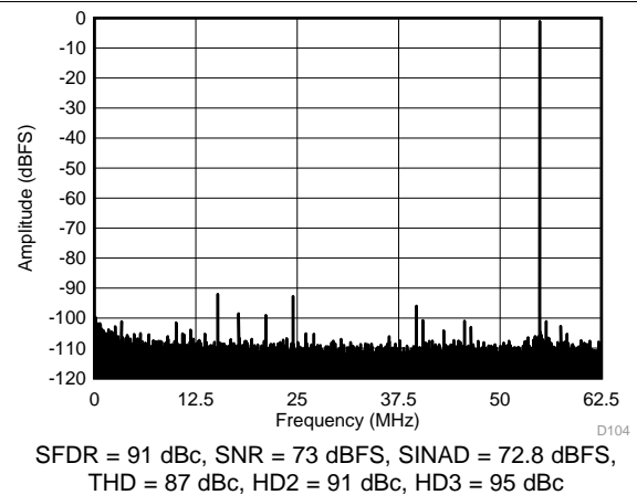
Figure 103. FFT for 70-MHz Input Signal (Dither Off)
