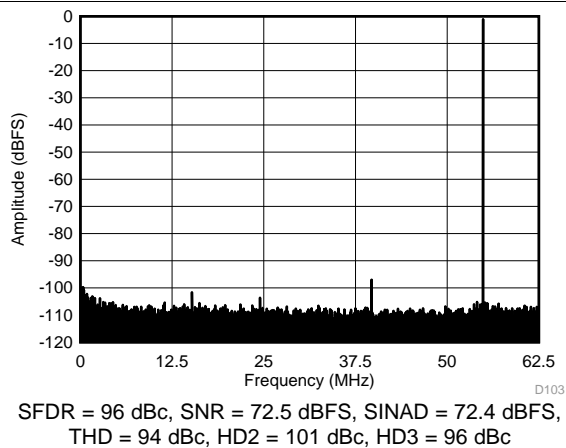
Figure 102. FFT for 70-MHz Input Signal (Dither On)
