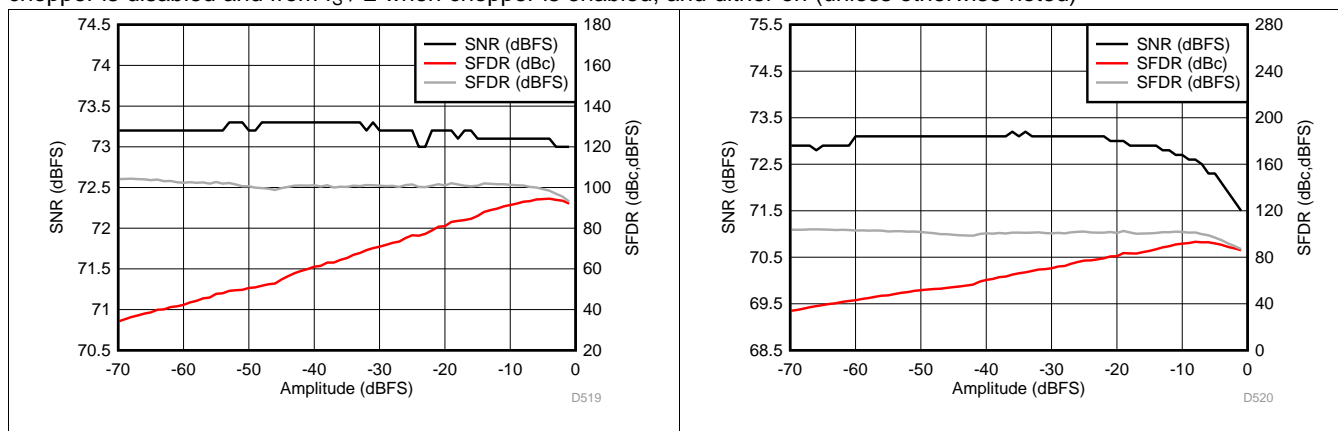
Figure 52. Performance vs Input Amplitude (30 MHz)
