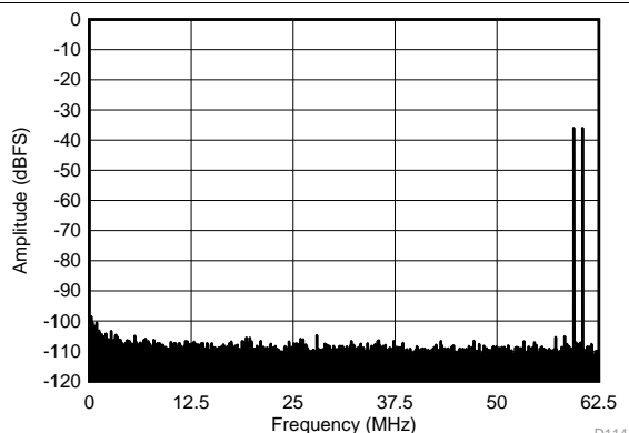
f_{IN1} = 185\text{ MHz} , f_{IN2} = 190\text{ MHz} , \text{IMD3} = 104\text{ dBFS} , each tone at -36\text{ dBFS}
