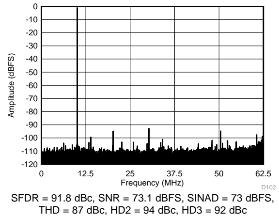
Figure 101. FFT for 10-MHz Input Signal (Chopper On, Dither Off)
