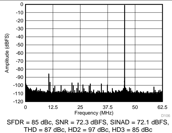
Figure 105. FFT for 170-MHz Input Signal (Dither Off)
