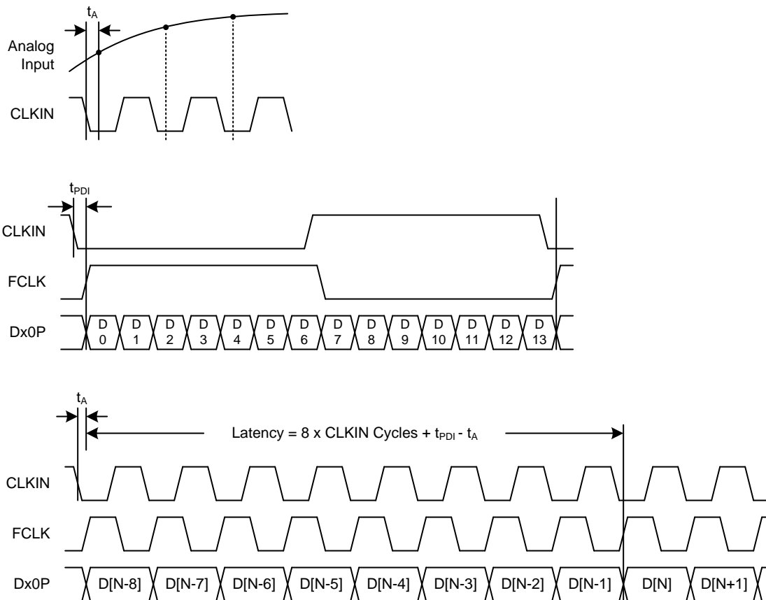
Figure 141. Latency Timing Diagram
