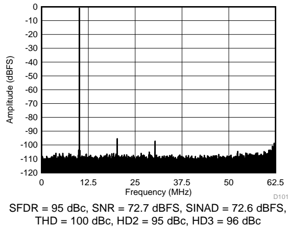
Figure 100. FFT for 10-MHz Input Signal (Chopper On, Dither On)
