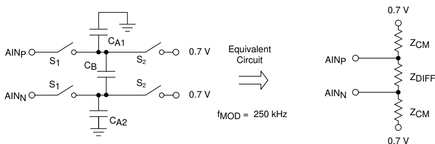
Figure 7-5. Simplified Analog Input Circuit
