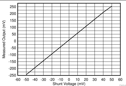
Figure 9-7. Measured Output vs Shunt Voltage ( V_{\text{SHUNT}} )
