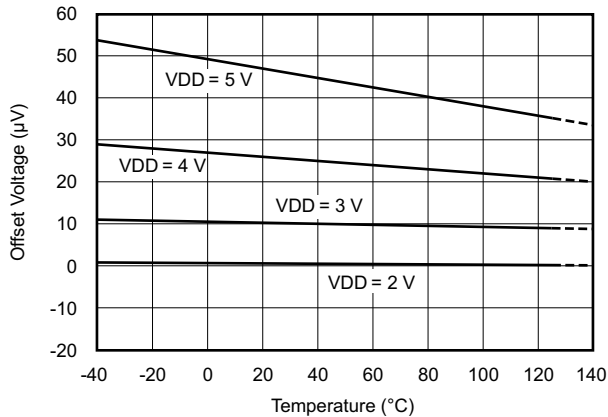
Figure 5-5. Differential Offset Error vs Temperature
