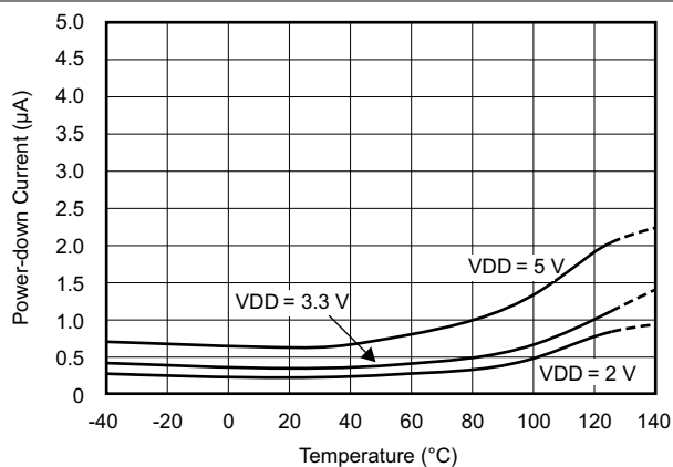
Figure 5-3. Power-Down Current vs Temperature
