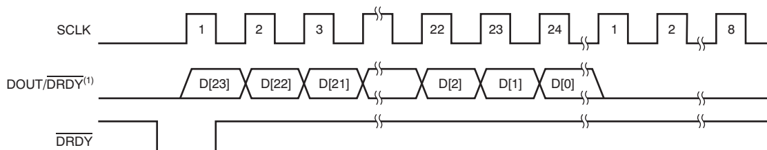
Figure 73. Data Retrieval with the \overline{\text{DRDY}} MODE Bit = 0 (Disabled)
