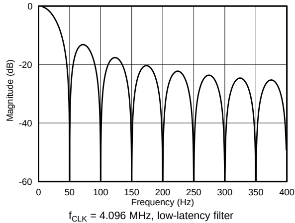
Figure 60. Low-Latency Filter Frequency Response, Data Rate = 50 SPS
