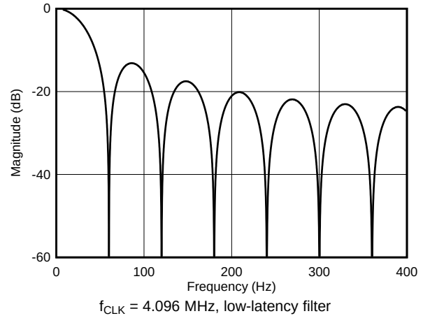
Figure 61. Low-Latency Filter Frequency Response, Data Rate = 60 SPS
