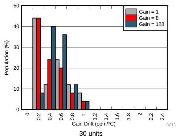
Figure 16. Gain Error Drift Distributions
