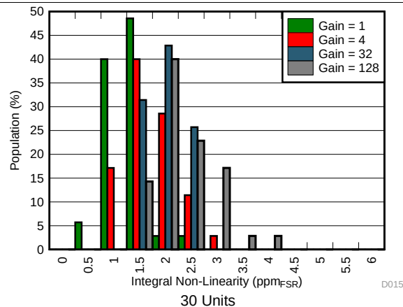
Figure 28. Integral Nonlinearity Distribution
