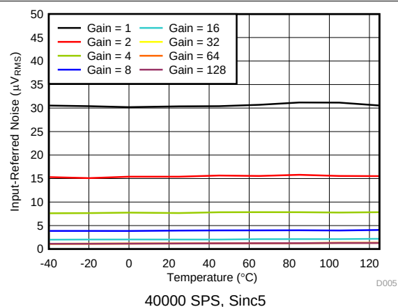
Figure 20. Noise vs Temperature
