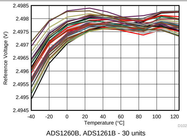
Figure 30. Voltage Reference vs Temperature
