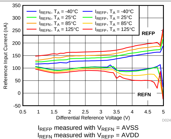
Figure 32. Reference Input Current vs Reference Voltage
