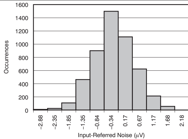
Figure 4. Noise Histogram
