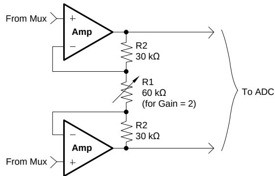
Figure 21. PGA Implementation
