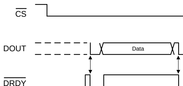
Figure 38. Using DOUT as \overline{\text{DRDY}}
