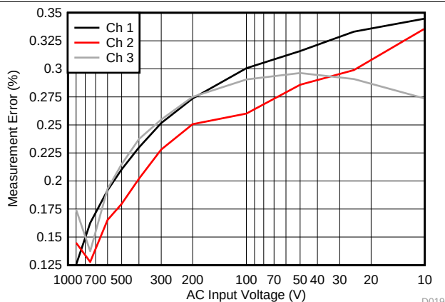
Figure 62. Input Voltage vs ADC Measurement Error: 4-V Reference
