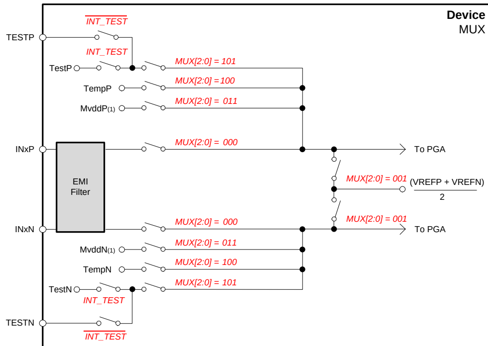
Figure 16. Input Multiplexer Block for One Channel
