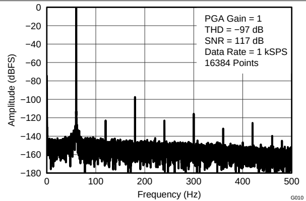
Figure 10. THD FFT Plot
