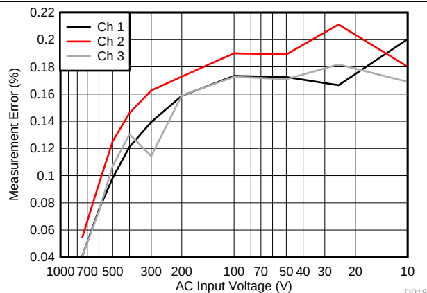
Figure 61. Input Voltage vs ADC Measurement Error: 2.4-V Reference
