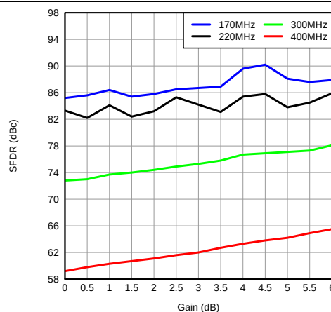
Figure 14. SFDR Across Gain and Input Frequency
