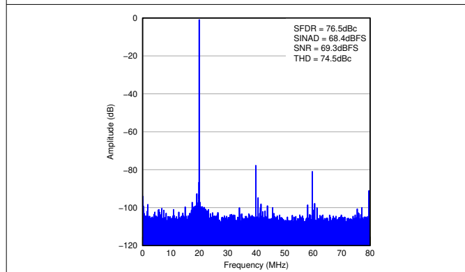
Figure 7-8. FFT for 300-MHz Input Signal
