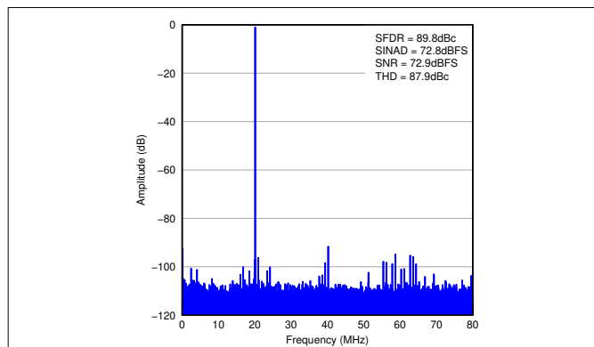
Figure 7-6. FFT for 20-MHz Input Signal
