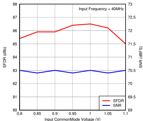
Figure 7-81. Performance vs Input Common-Mode Voltage
