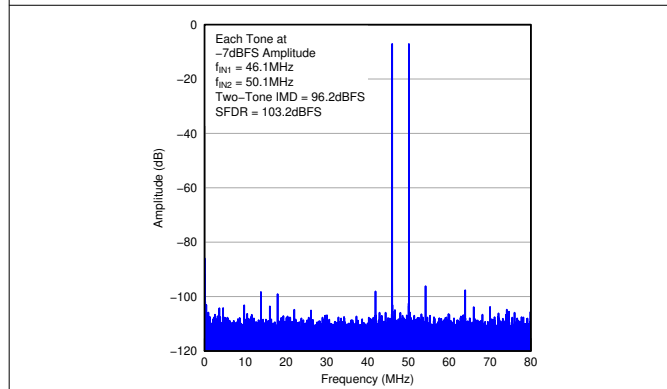
Figure 7-10. FFT for Two-Tone Input Signal
