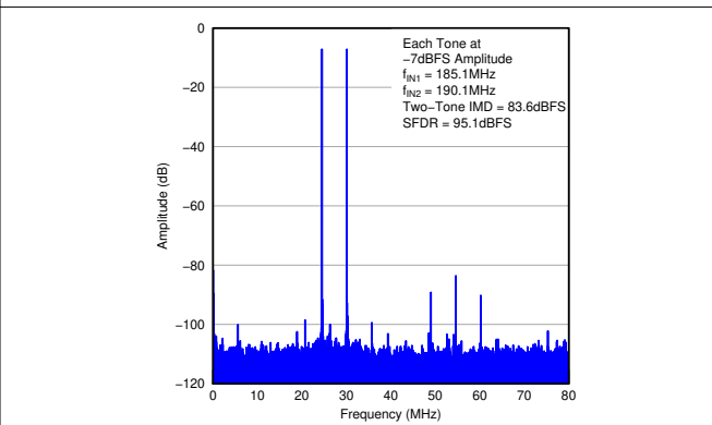
Figure 7-9. FFT for Two-tone Input Signal
