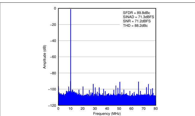
Figure 7-7. FFT for 170-MHz Input Signal
