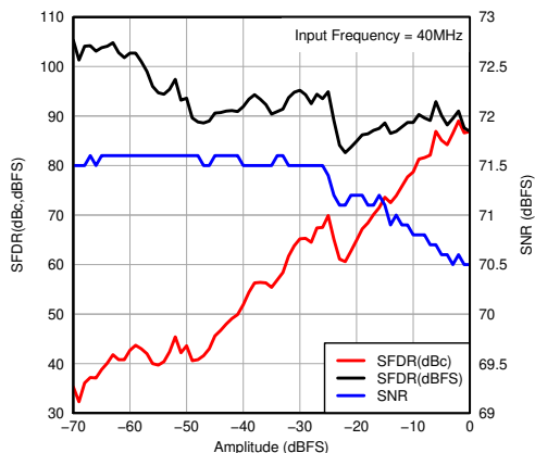
Figure 7-79. Performance vs Input Amplitude
