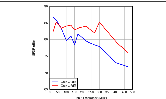
Figure 7-11. SFDR vs Input Frequency
